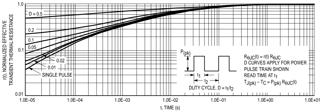
Figure 13. Thermal Response
