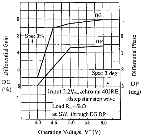
Differential Gain/Differential
