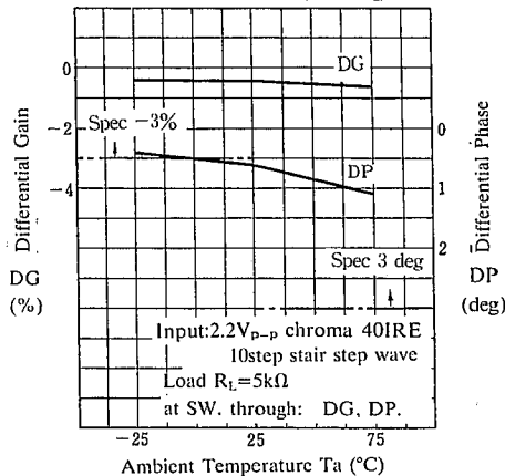
Differential Gain/Differential Phase
