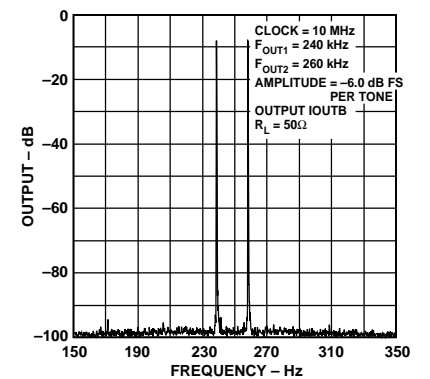
Figure 20. Intermodulation Distortion
