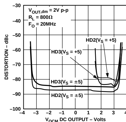
Figure 10. Harmonic Distortion vs. V_{OCM}
