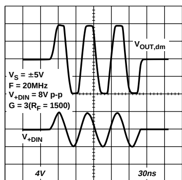
Figure 23. Output Overdrive
