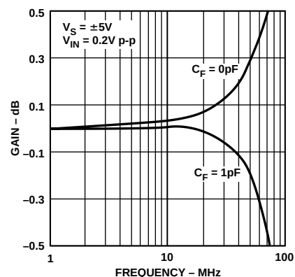
Figure 4. 0.1 dB Flatness vs. Frequency
