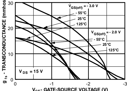
Transfer Characteristics
