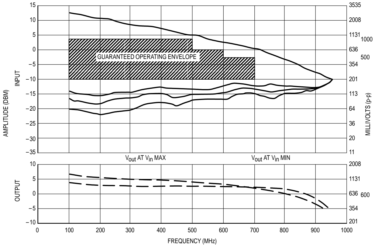
Figure 1. Guaranteed Range of Operation (Temp = 75°C, 5 Devices, VCC = 2.0V, VEE = -3.2V, VBias = 0.710V)
