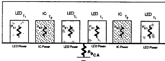
FIGURE 5. THERMAL MODEL
