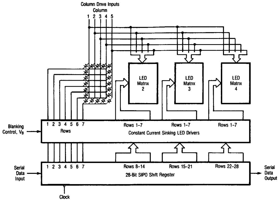
FIGURE 4. BLOCK DIAGRAM
