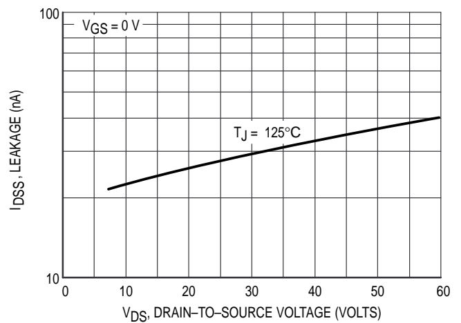
Figure 6. Drain-To-Source Current versus Voltage
