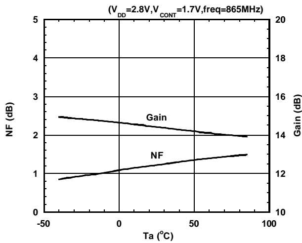
NF, Gain vs. Ta
