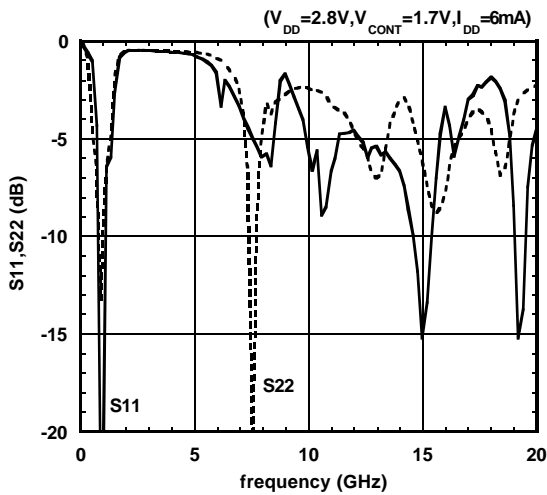
S11,S22 vs. frequency
