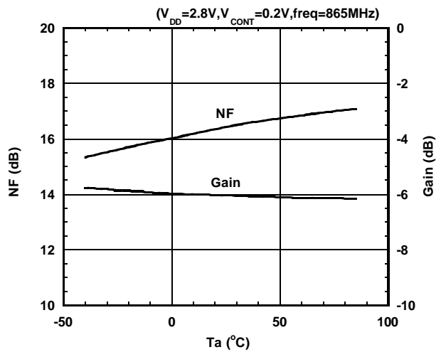
NF, Gain vs. Ta
