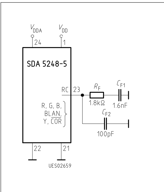
Test Circuit 3
