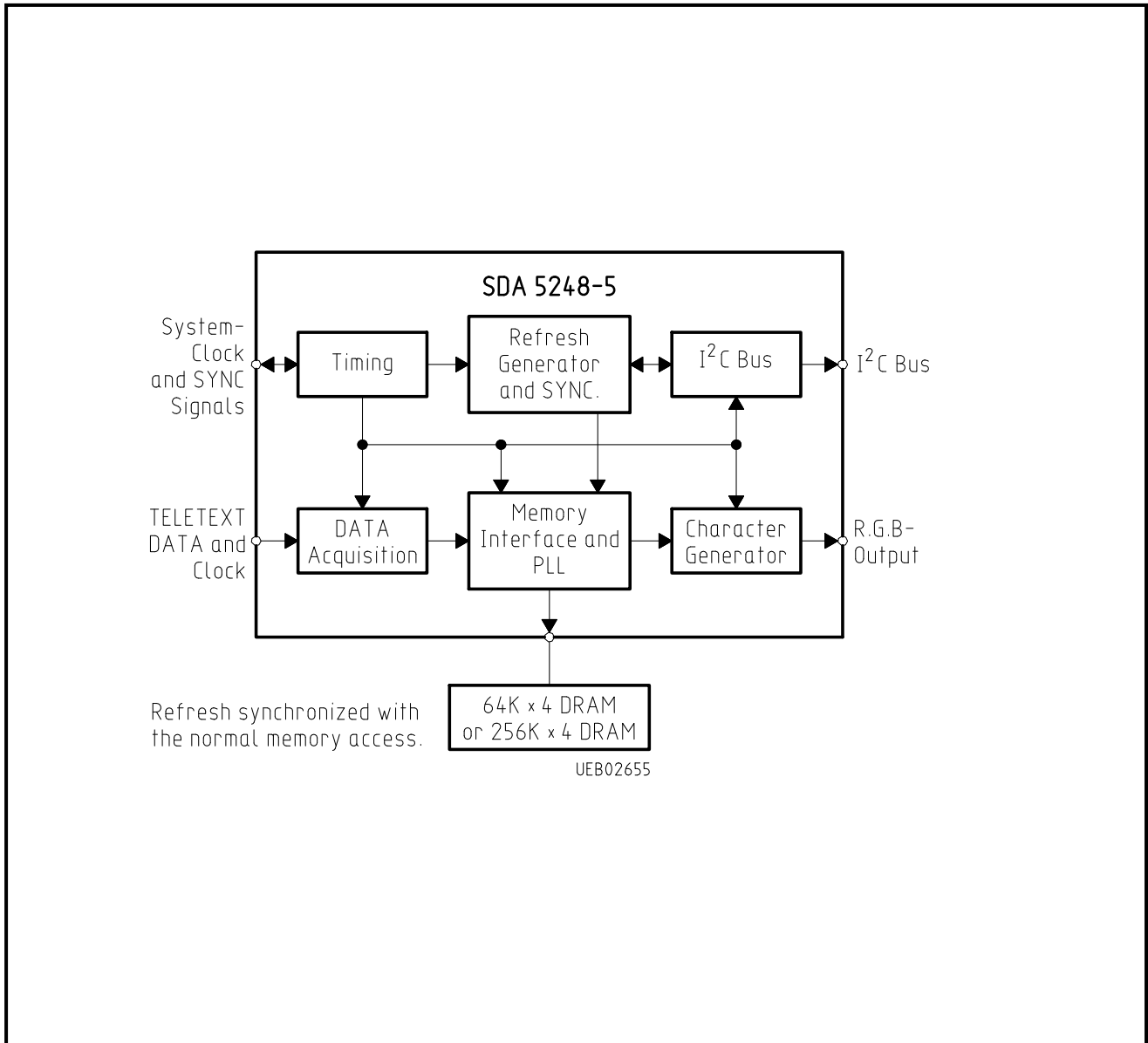
Block Diagram Teletext Processor with DRAM Interface
