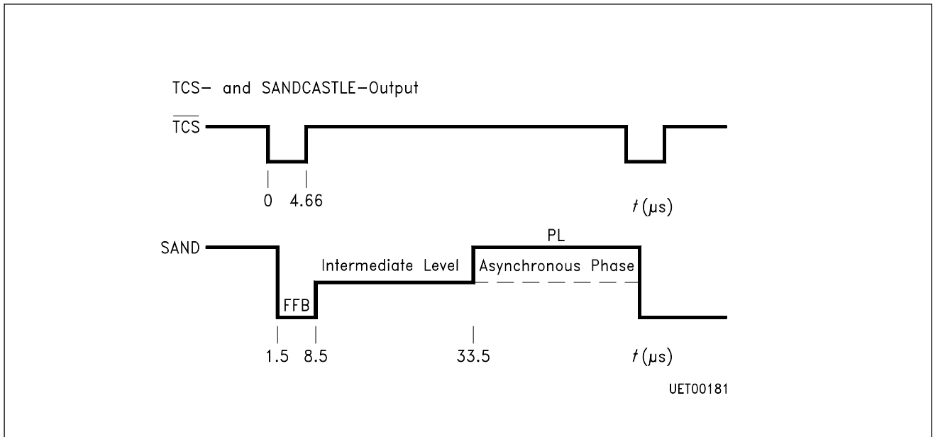
Timing Diagram 3 TCS and SANDCASTLE-Output
