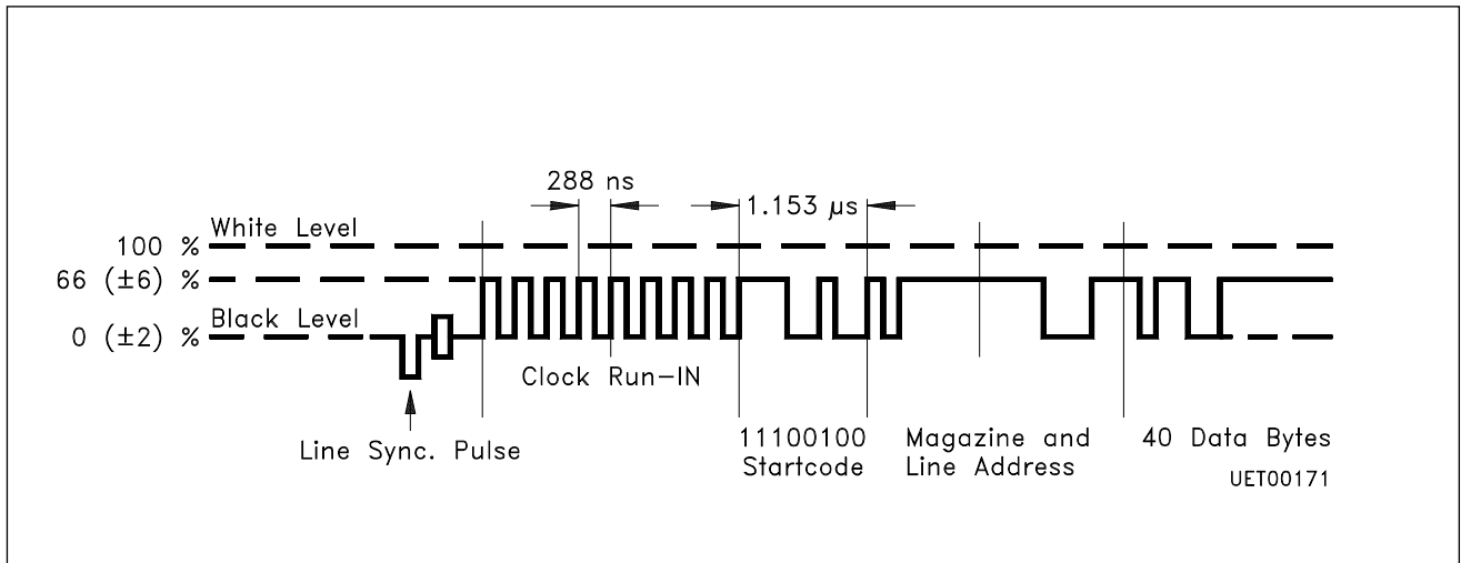
Diagram 1 Teletext Input Signal (Line 2 to 22 and 315 to 335)
