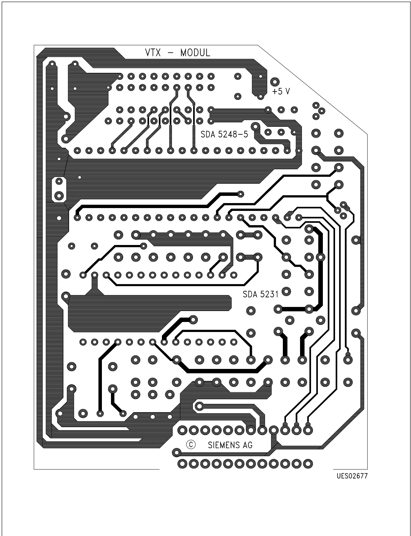
Layout / Plug-In Location Plan
