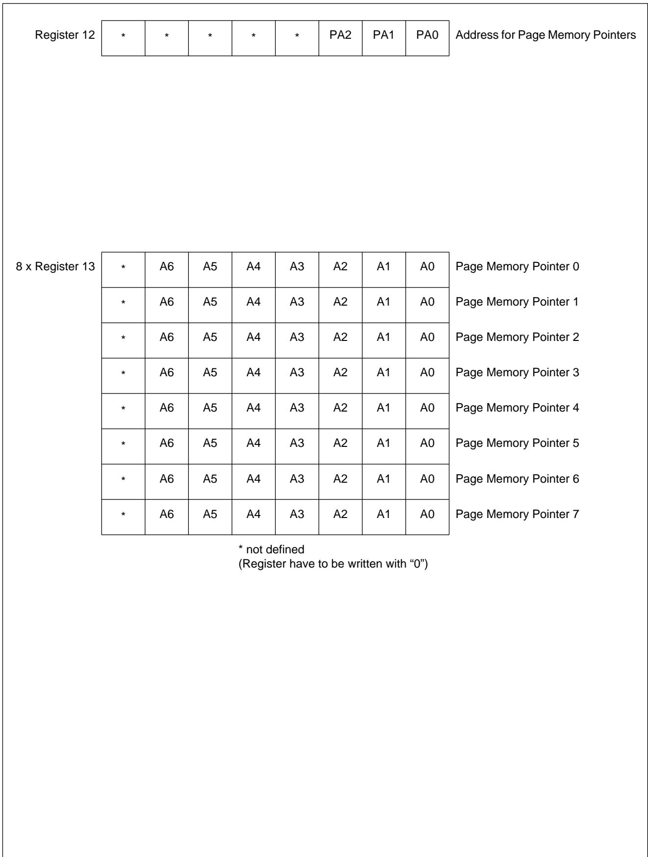
Diagram 7 Register Configuration
