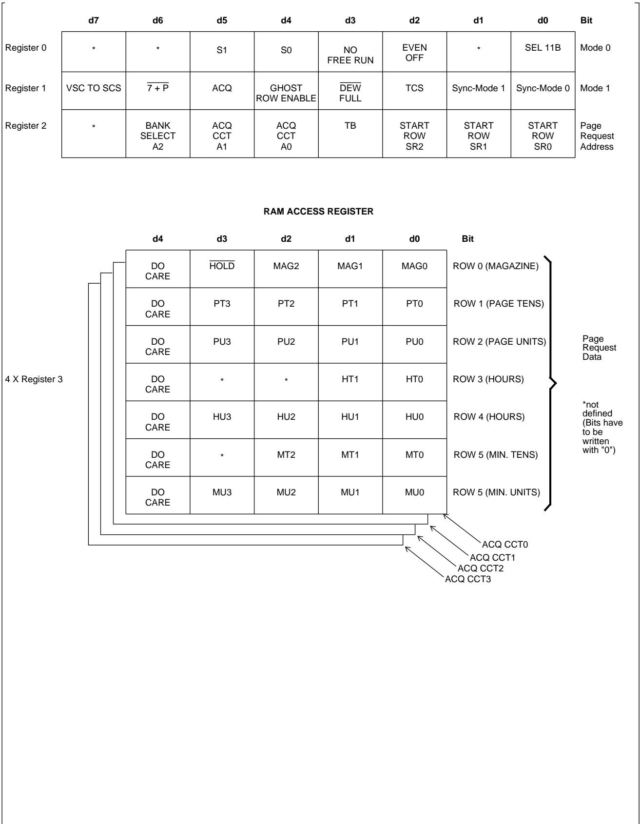
Diagram 5 Register Configuration
