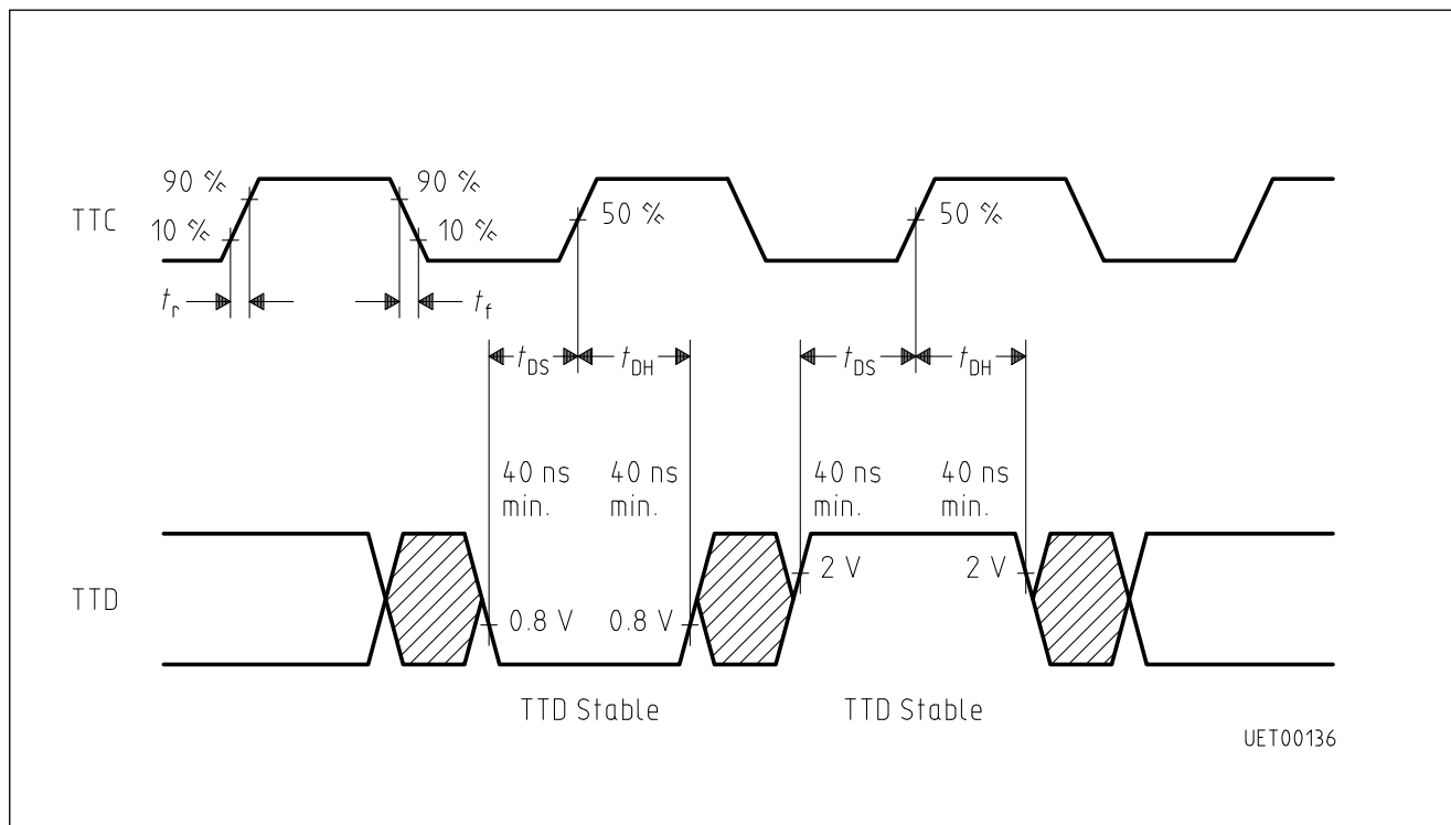
Timing Diagram 2 Input Signals TTC and TTD
