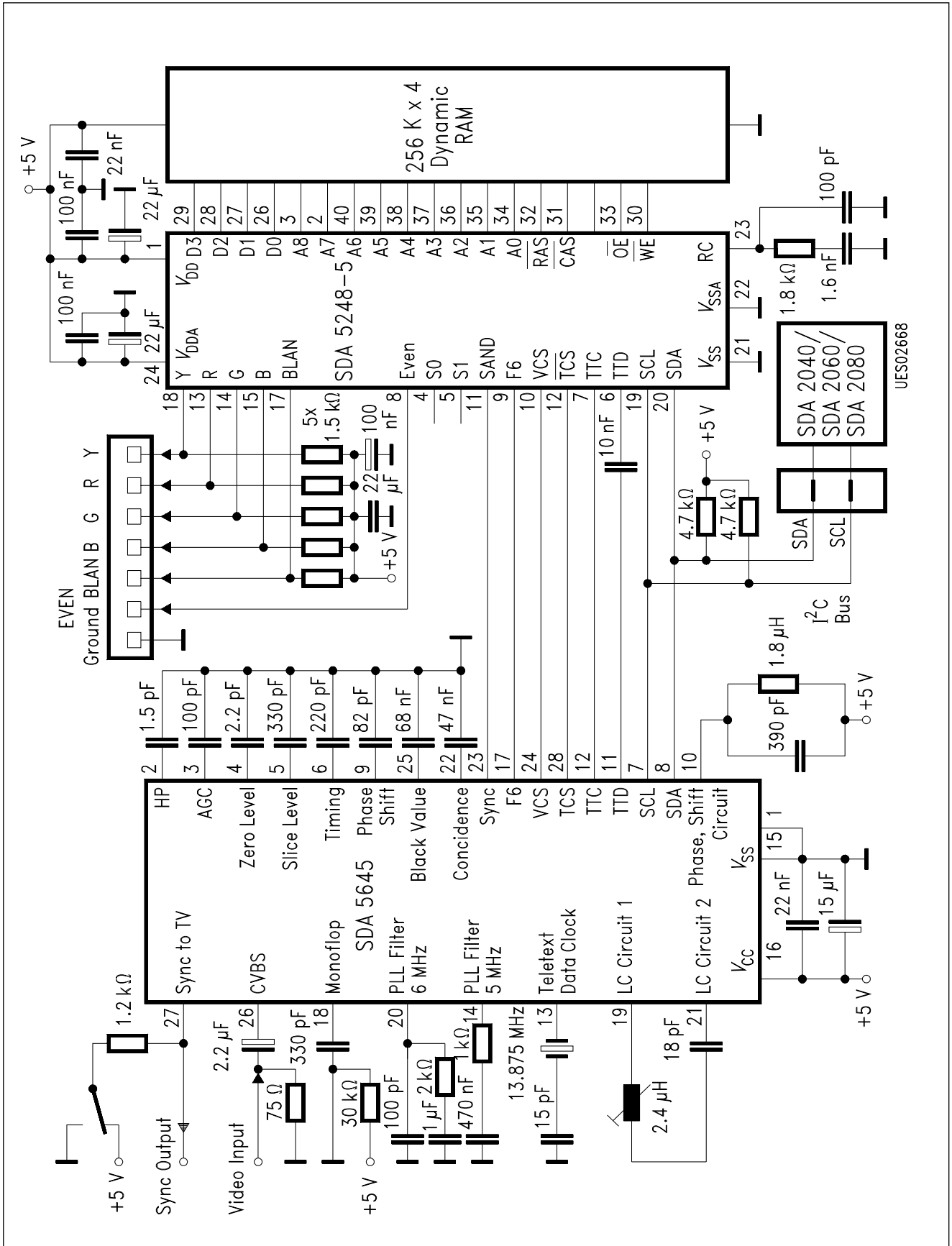
Application Circuit 5
