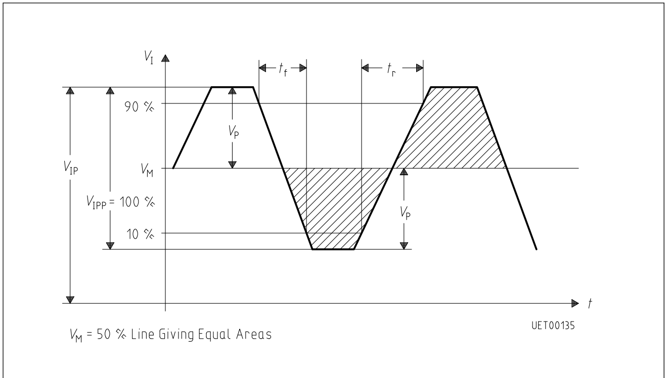
Timing Diagram 1 Input Signals TTC and F6
