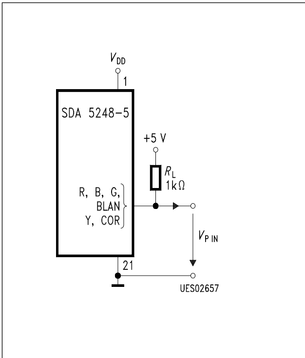
Test Circuit 1
