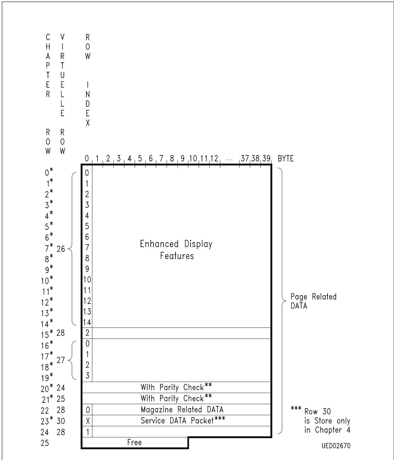
Diagram 3 Virtual Page (Ghost Rows)
