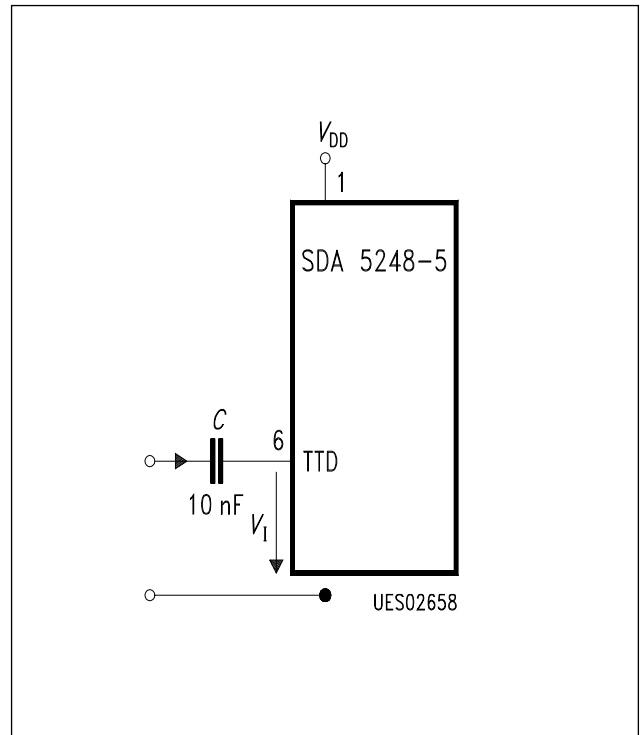
Test Circuit 2
