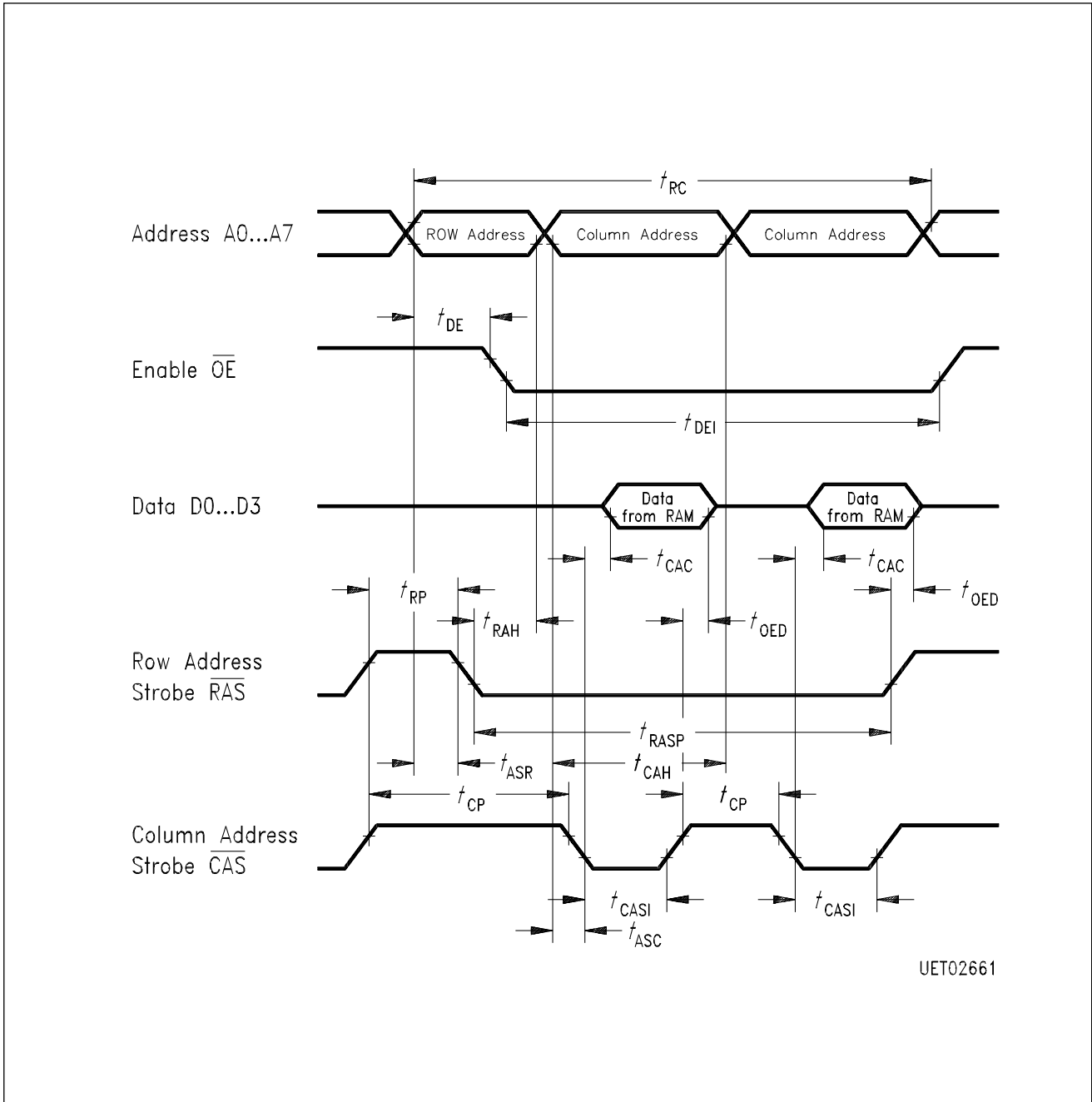
Timing Diagram 5b Data Transfer with External Page Memory Dynamic Memory 64 K x 4 or 256 K x 4 Memory Read (Page Mode Read Cycle)
