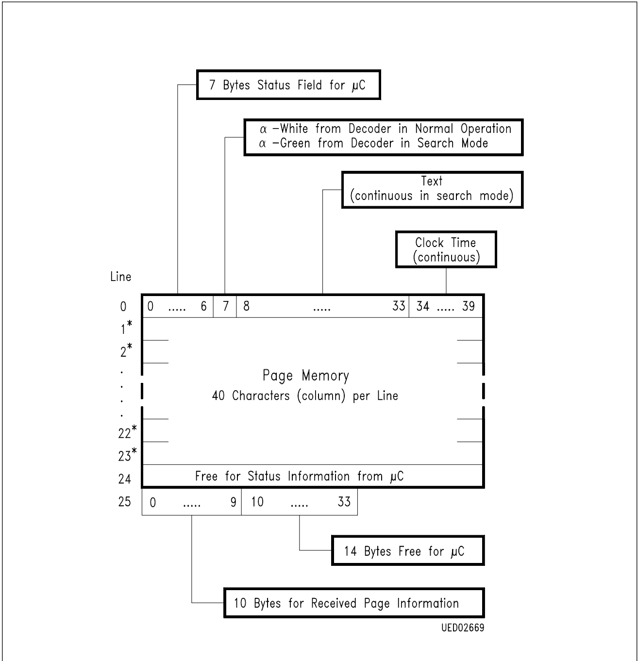
Diagram 2 Page Memory Organization
