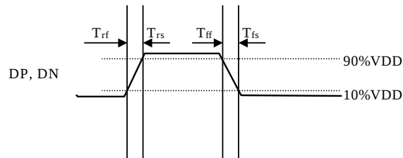
Figure 3. Rise/Fall Time
