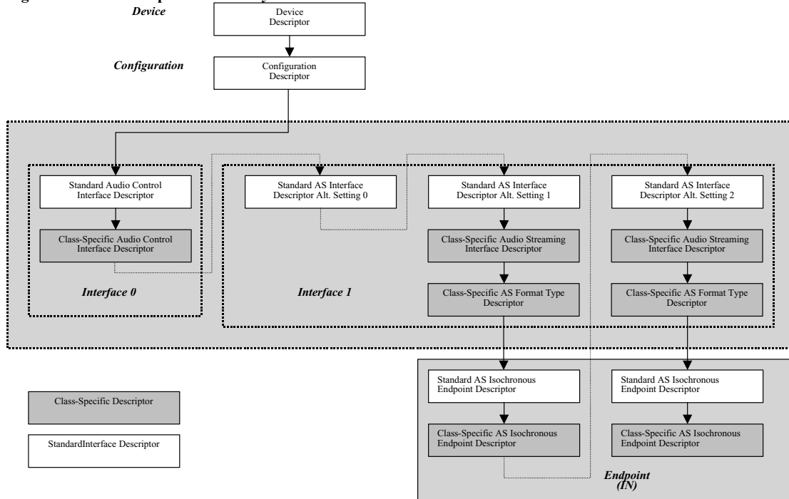
Figure 6. Descriptor Hierarchy
