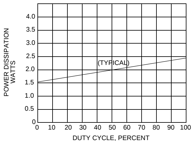
Figure 6 Power Dissipation vs. Duty Cycle (Per Channel)
