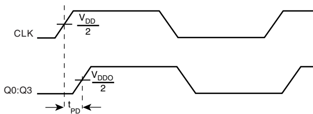
PROPAGATION DELAY
