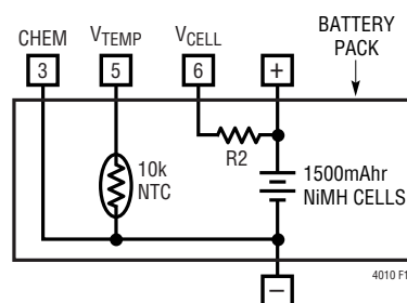
Figure 11. NiMH Battery Pack Indicating Number of Cells
