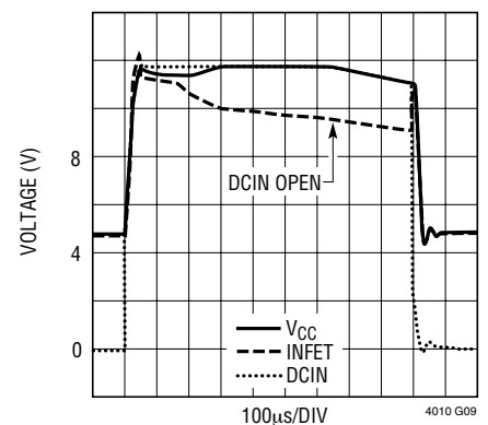
PowerPath Switching
