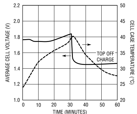
Typical NiMH Charge at 1.25C
