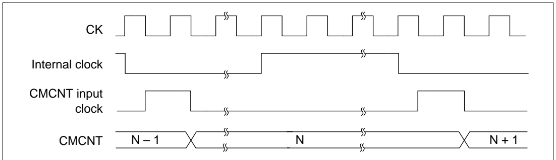
Figure 17.3 Count Timing
