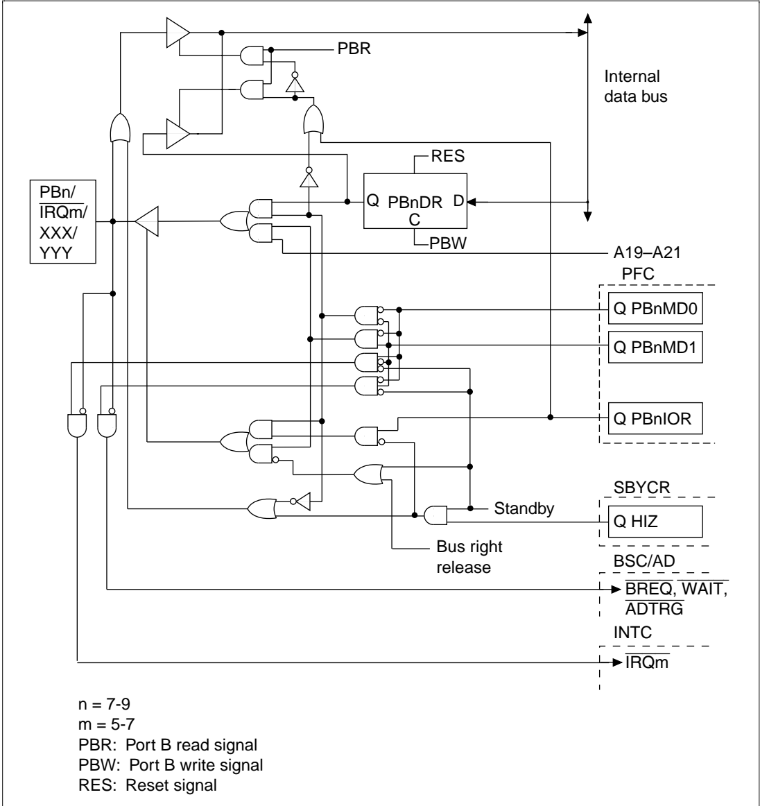
Figure B.20 \overline{\text{PBn}}/\overline{\text{IRQm}}/\text{XXX}/\text{YYY} Block Diagram
