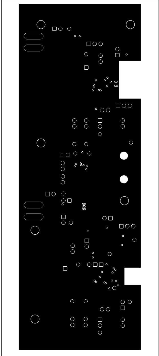
Figure 7. MAX3735 EV Kit PC Board Layout—Ground Plane
