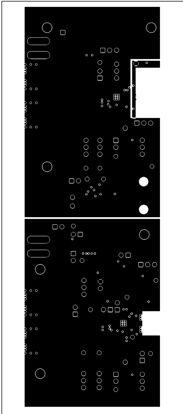
Figure 8. MAX3735 EV Kit PC Board Layout—Power Plane
