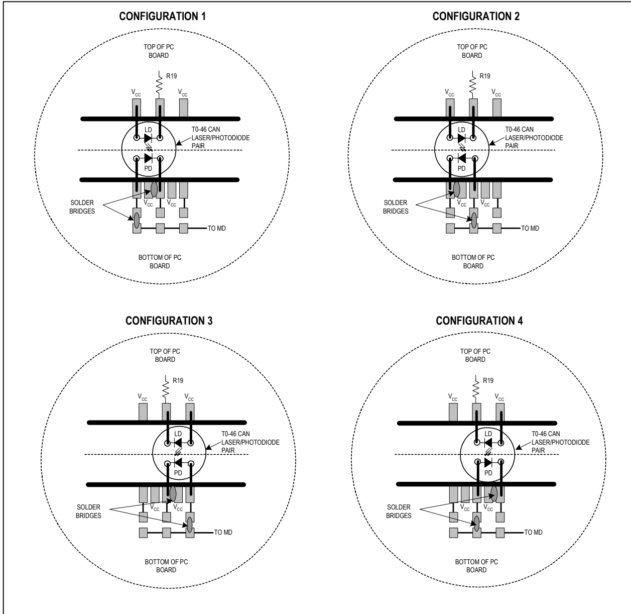
Figure 1. Attachment of Laser Diode/Monitor Diode to the MAX3735 EV Kit
