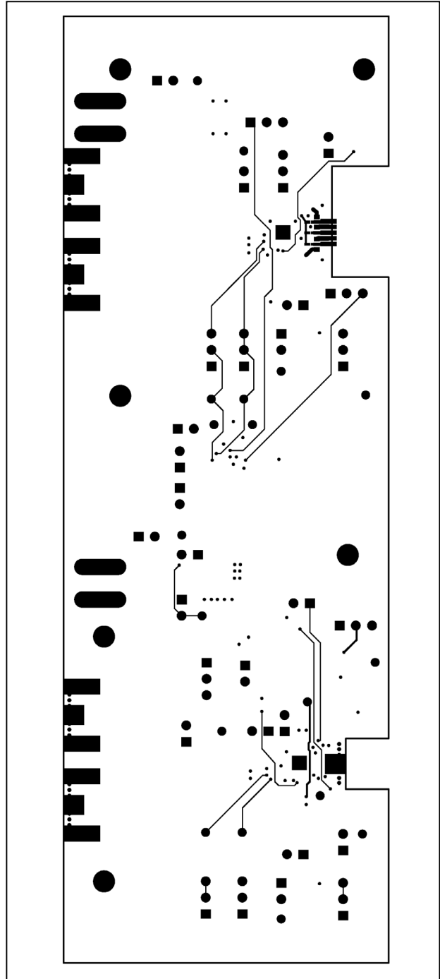
Figure 9. MAX3735 EV Kit PC Board Layout—Solder Side
