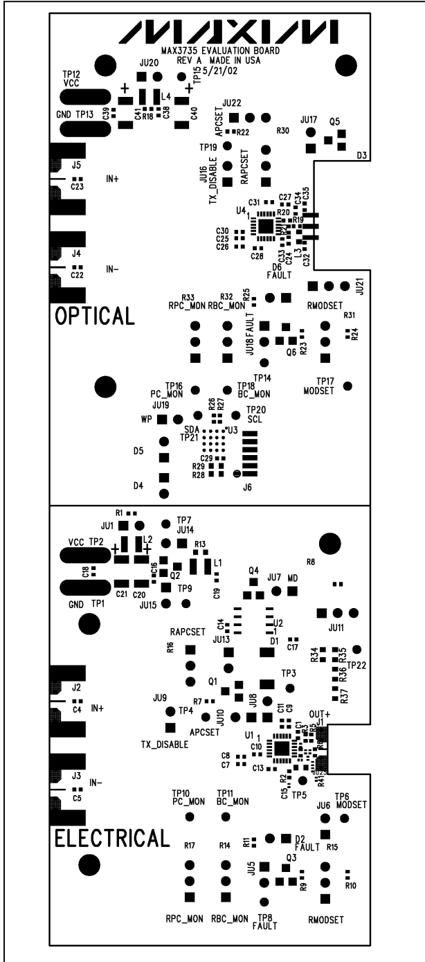
Figure 4. MAX3735 EV Kit PC Component Placement Guide—Component Side
