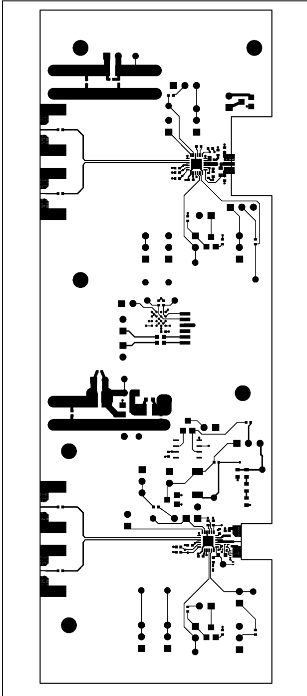
Figure 6. MAX3735 EV Kit PC Board Layout—Component Side
