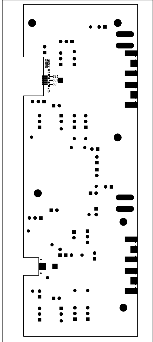
Figure 5. MAX3735 EV Kit PC Component Placement Guide—Solder Side
