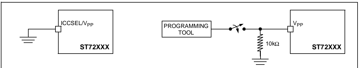
Figure 97. Two typical Applications with ICCSEL/V PP Pin 2)
