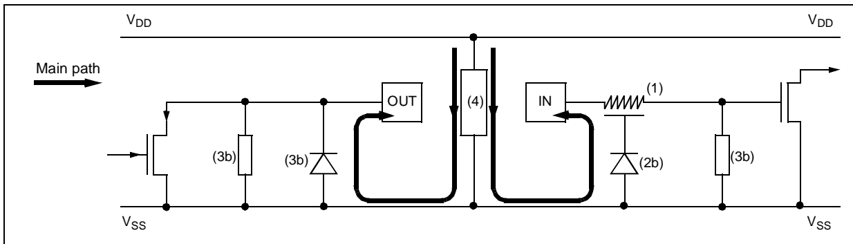
Figure 87. Multisupply Configuration
