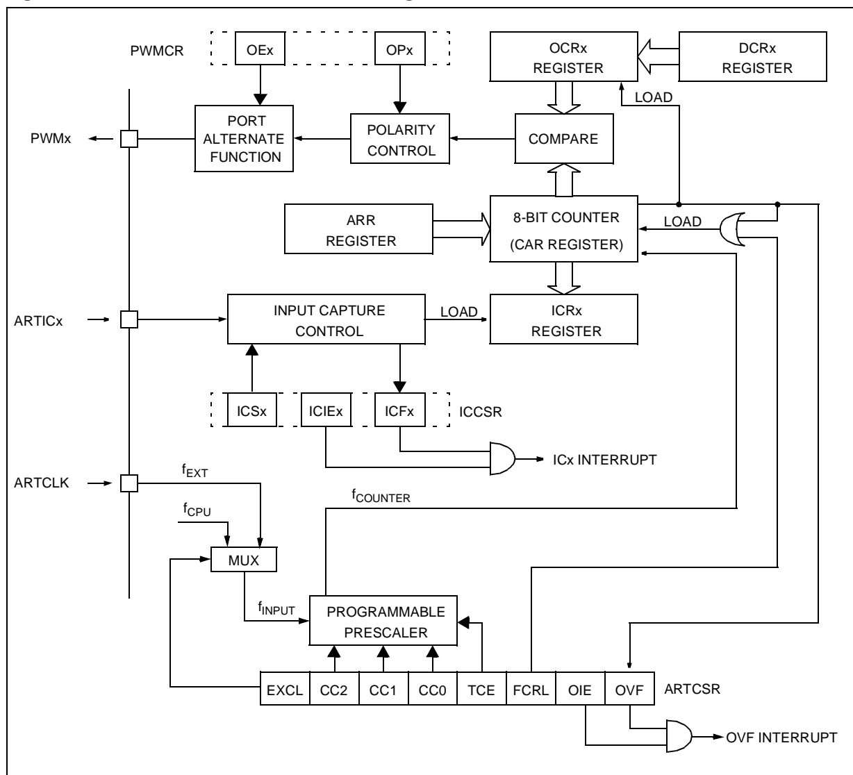
Figure 35. PWM Auto-Reload Timer Block Diagram
