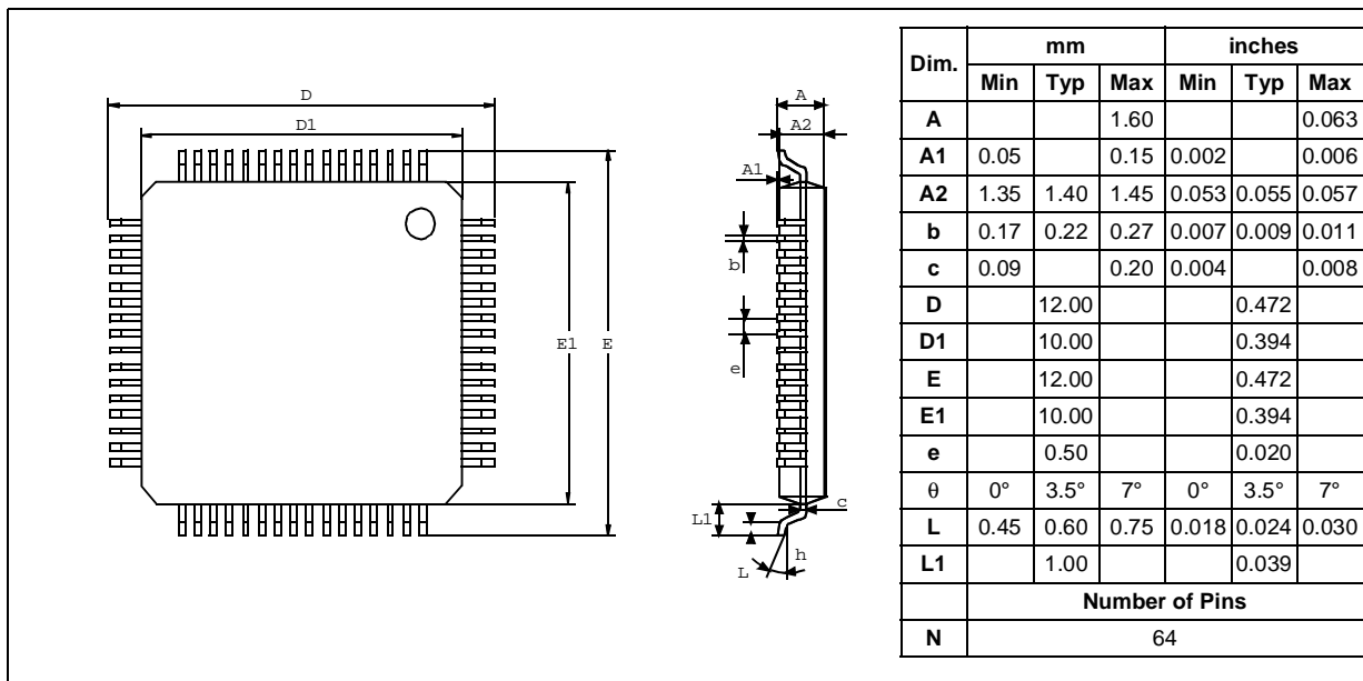
Figure 108. 64-Pin Thin Quad Flat Package
