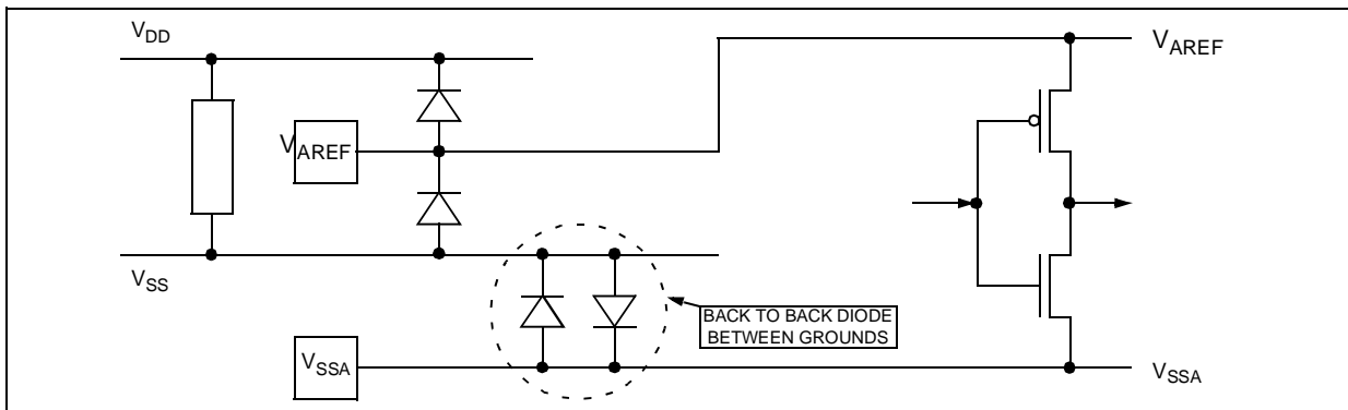
Figure 87. Multisupply Configuration
