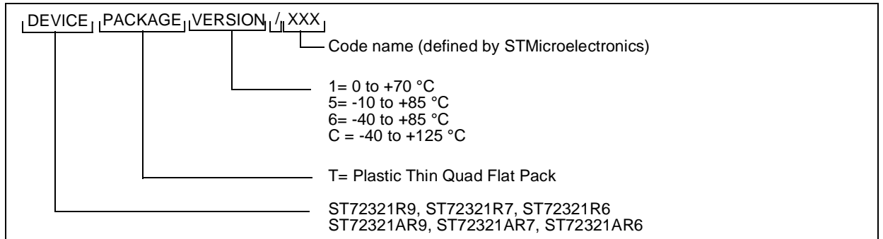
Figure 111. ROM Factory Coded Device Types
