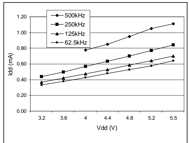
Figure 72. Typical I DD in SLOW vs. f CPU
