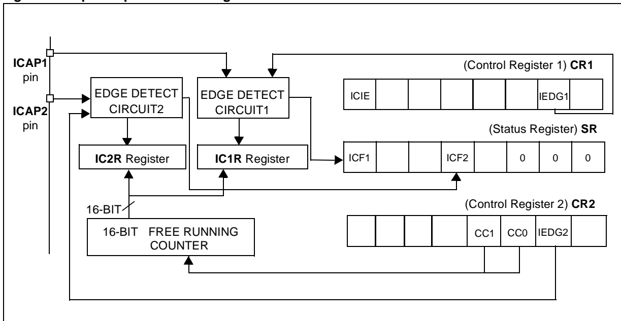
Figure 45. Input Capture Block Diagram
