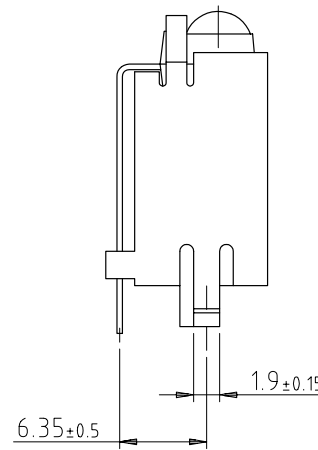
View "A"
