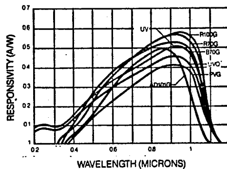
RESONSIVITY CURVES (TYPICAL)
