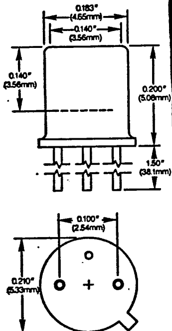
TO-18
