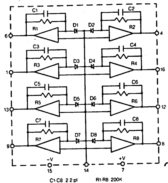
CONNECTION DIAGRAM FOR 7000POH08M
