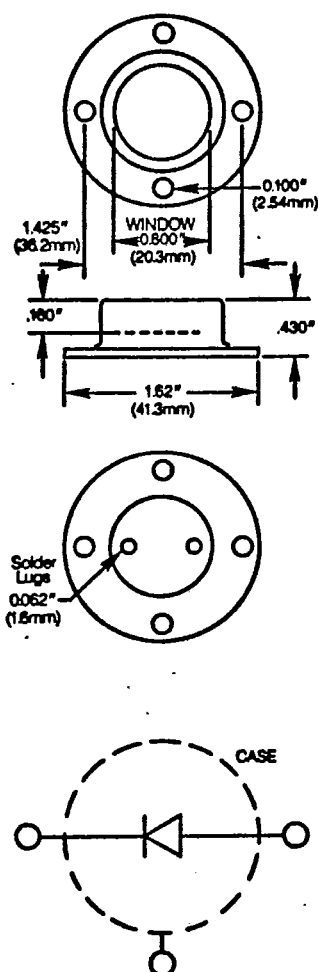
TO-3/3
