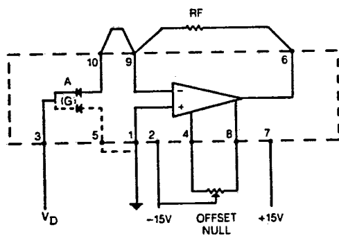
CONNECTION DIAGRAM FOR SINGLE ELEMENT OPTO-HYBRIDS
