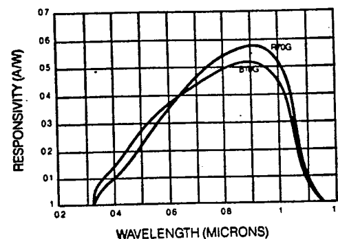
RESPONSIVITY CURVES (TYPICAL)
