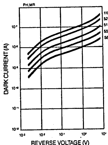
DARK CURRENT vs. VOLTAGE
