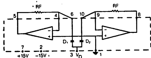
CONNECTION DIAGRAM FOR 25PDU0H74M
