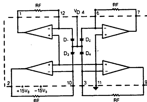
CONNECTION DIAGRAM FOR 45QUH08M
