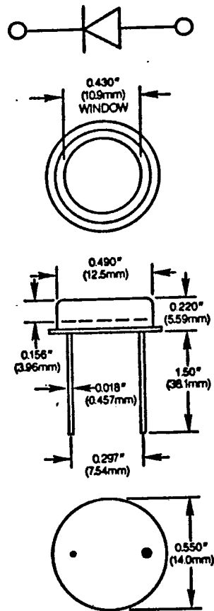
TO-8
