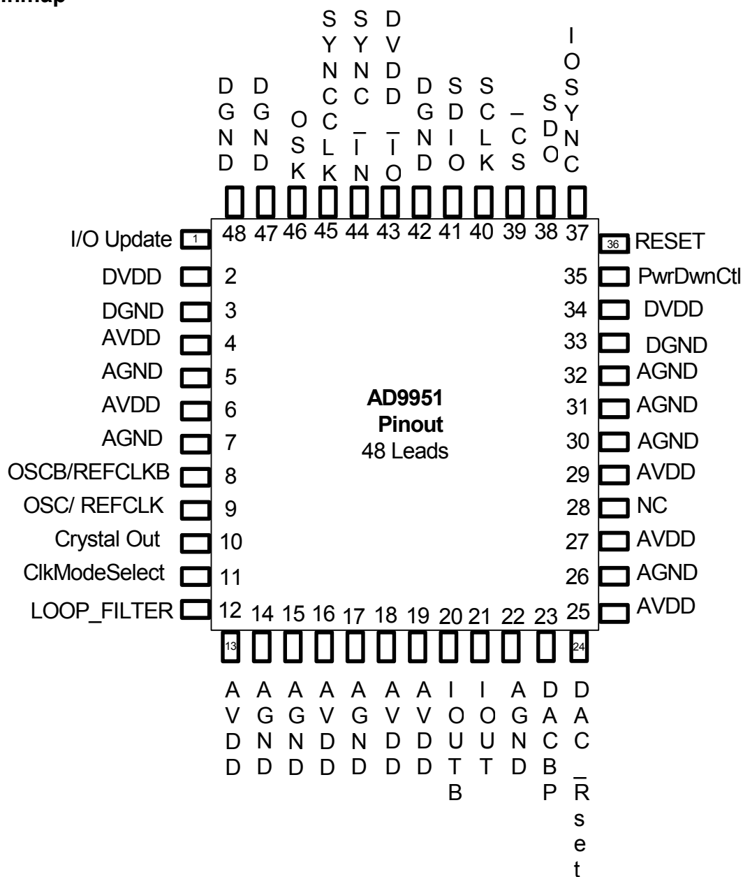
Figure 1 AD9951 Pinmap
