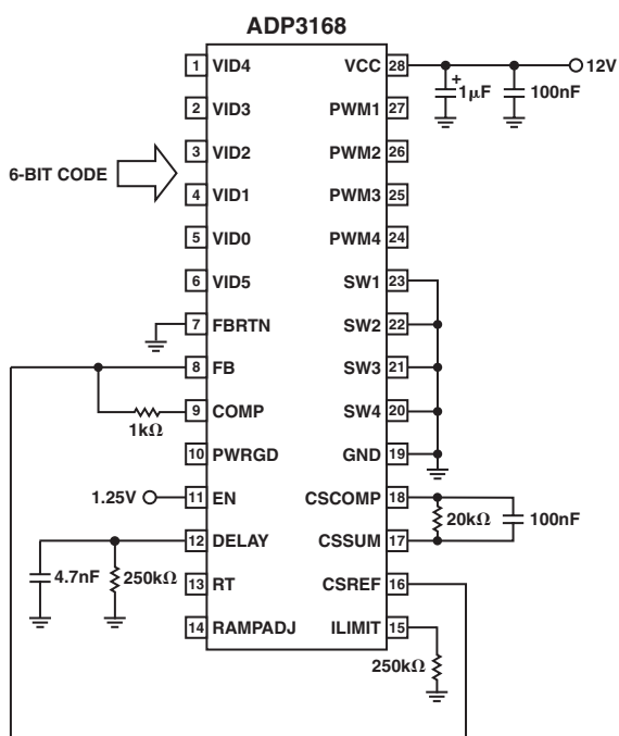
Test Circuit 3. Closed-Loop Output Voltage Accuracy
