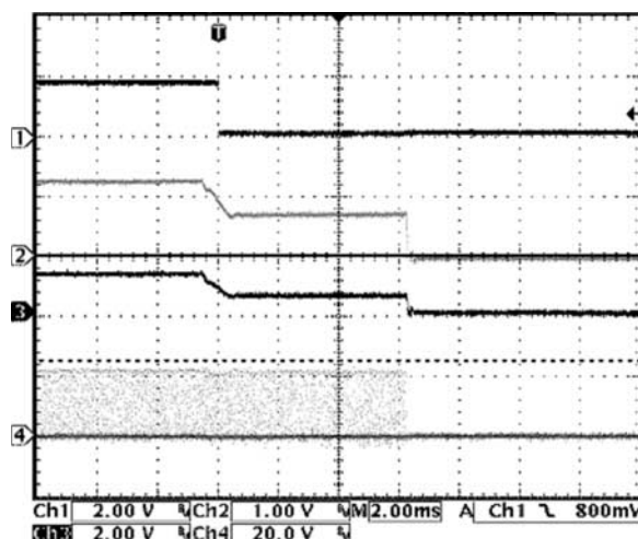
Figure 2. Overcurrent Latch-Off Waveforms, Circuit of Figure 4.
