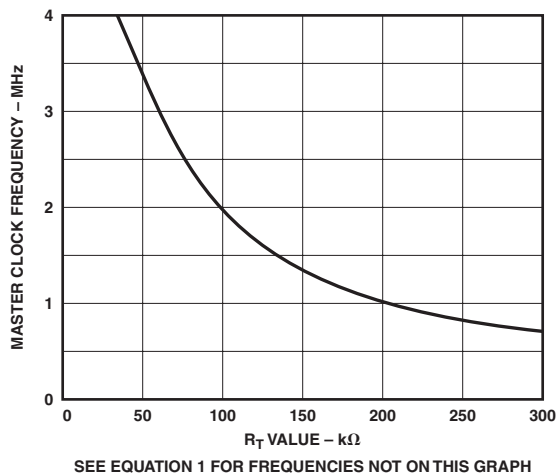
TPC 1. Master Clock Frequency vs. R_T
