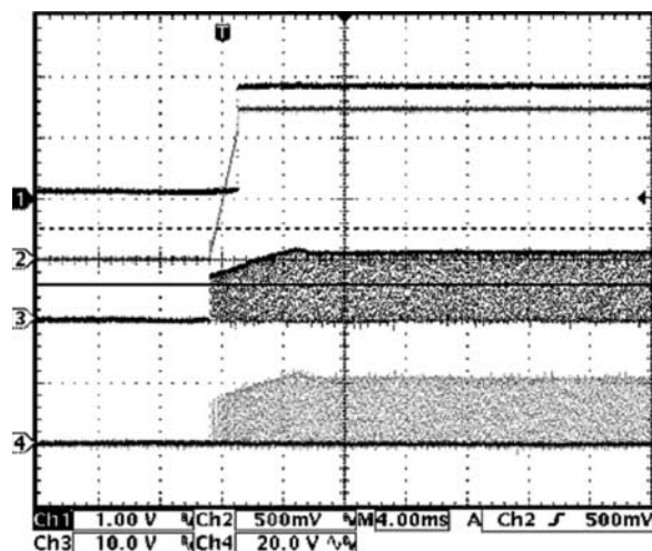
Figure 1. Start-Up Waveforms, Circuit of Figure 5.
