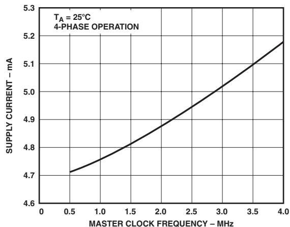
TPC 2. Supply Current vs. Master Clock Frequency
