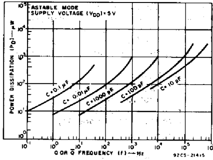
Fig. 26—Typical power dissipation vs. output frequency ( V_{DD} = 5 V).
