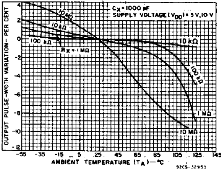
Fig. 24—Typical output pulse-width variations vs. ambient temperature.
