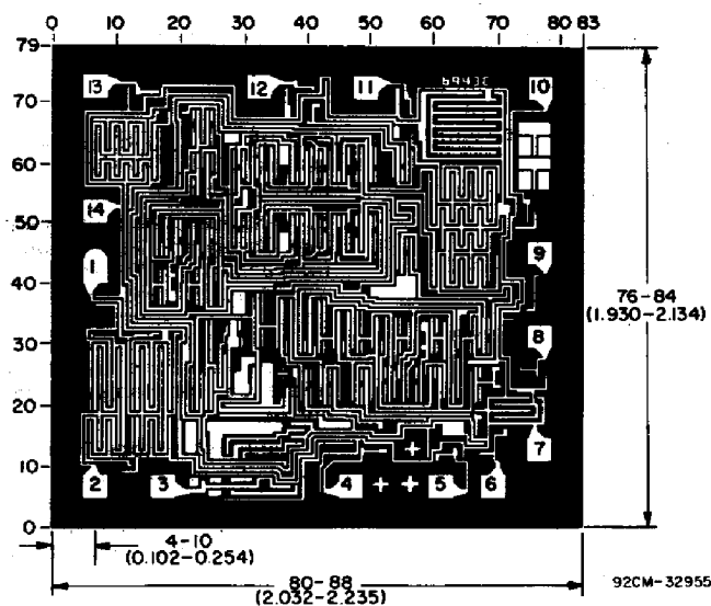
Chip dimensions and pad layout for CD4047B
