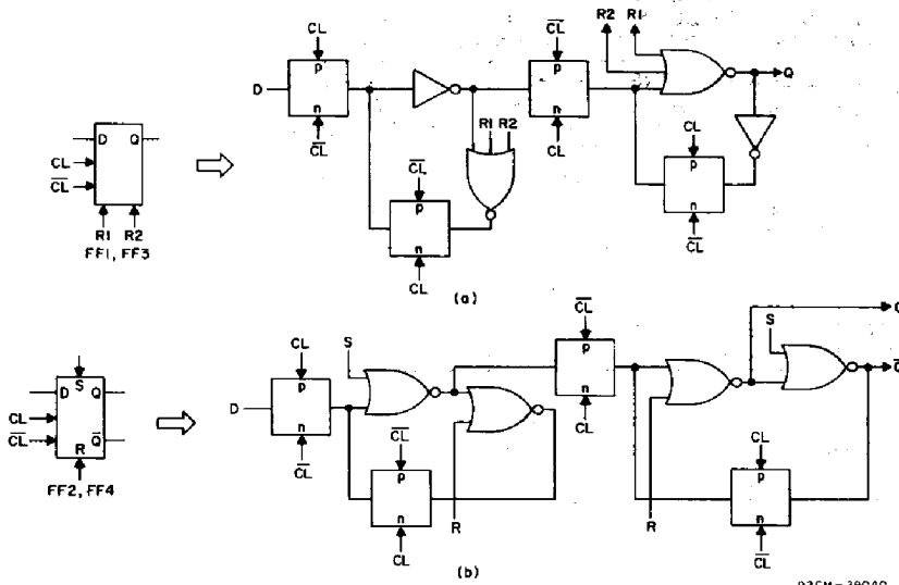
Fig. 3—Detail logic diagram for flip-flops FF1 and FF3 (a) and for flip-flops FF2 and FF4 (b).
