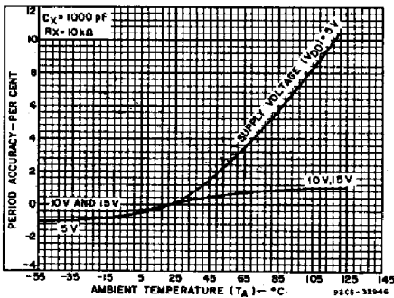
Fig. 17—Typical astable oscillator or Q, \bar{Q} period accuracy vs. ambient temperature (high-frequency).
