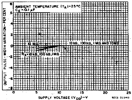
Fig. 20—Typical output pulse-width variations vs. supply voltage.
