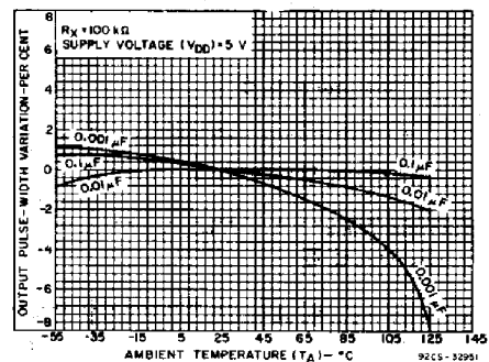
Fig. 22—Typical output pulse-width variations vs. ambient temperature.
