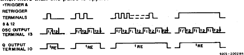
Fig. 34—Retrigger-mode waveforms.
