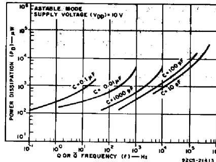
Fig. 27—Typical power dissipation vs. output frequency ( V_{DD} = 10 V).
