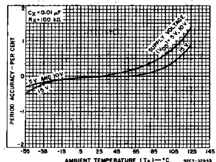
Fig. 16—Typical astable oscillator or Q, \bar{Q} period accuracy vs. ambient temperature (medium frequency).
