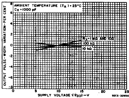
Fig. 21—Typical output pulse-width variations vs. supply voltage.
