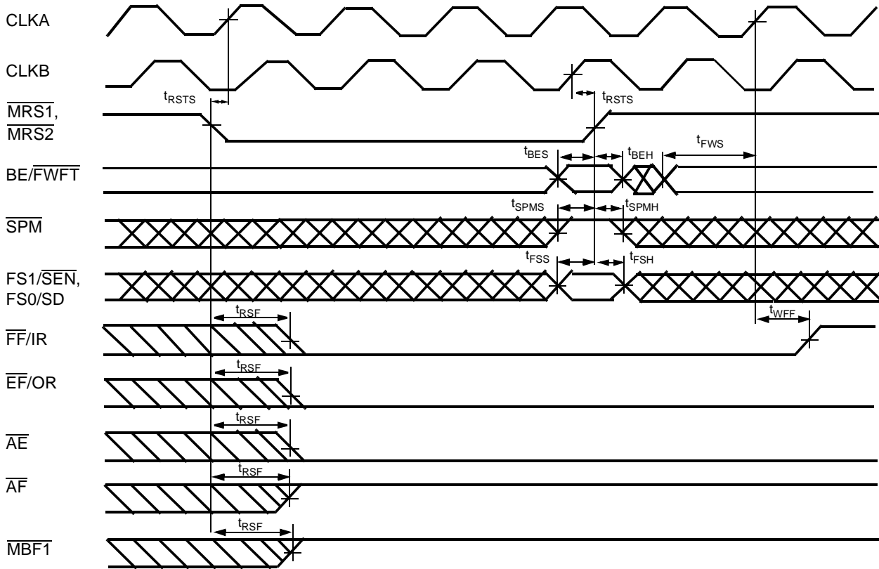
Master Reset Loading X and Y with a Preset Value of Eight [11]
