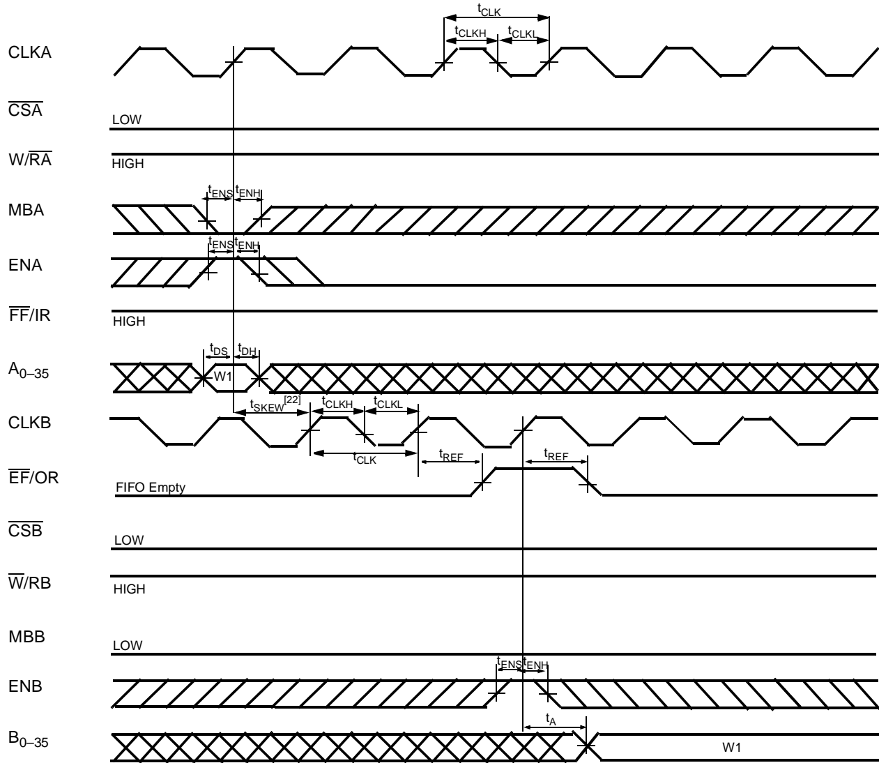
\overline{EF} Flag Timing and First Data Read Fall Through when FIFO is Empty (CY Standard Mode) [20]
