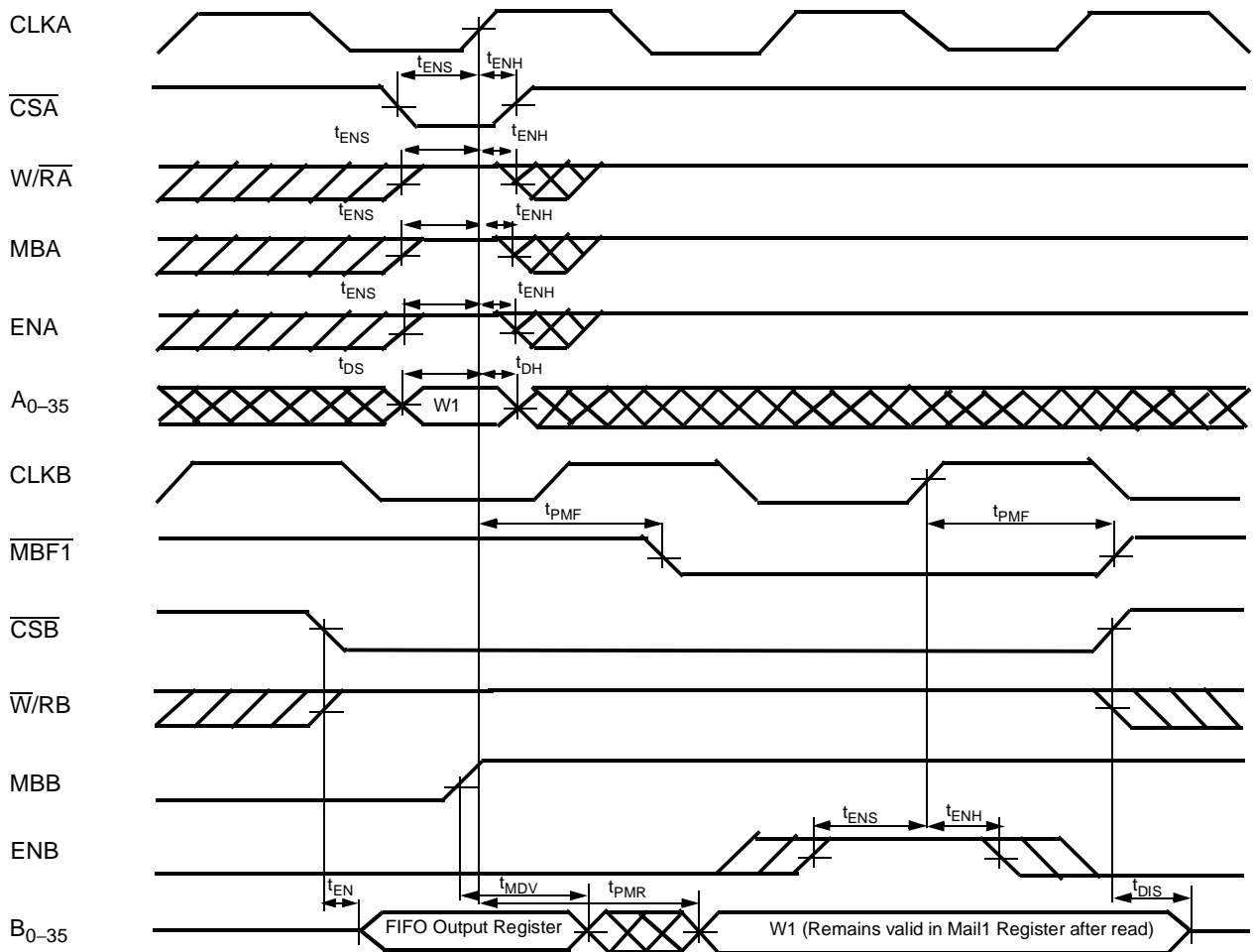
Timing for Mail1 Register and \overline{\text{MBF1}} Flag (CY Standard and FWFT Modes) [33]
