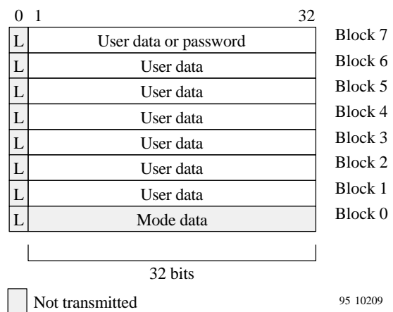
Figure 5. Memory map
