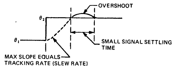
RESPONSE TO A STEP INPUT
