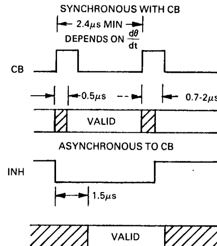
FIGURE 2. TIMING DIAGRAM
