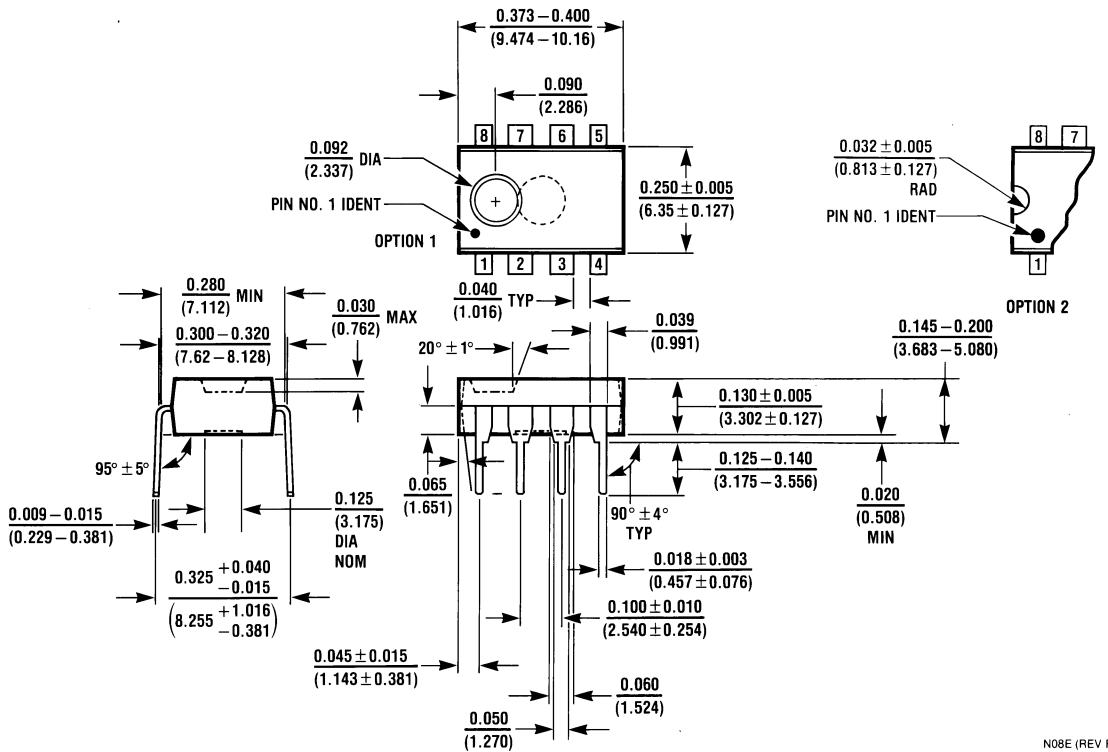
Order Number LM9022N NS Package Number N08E
