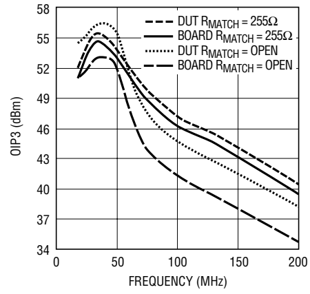
Figure 12. Typical OIP3 for Transformer Board
