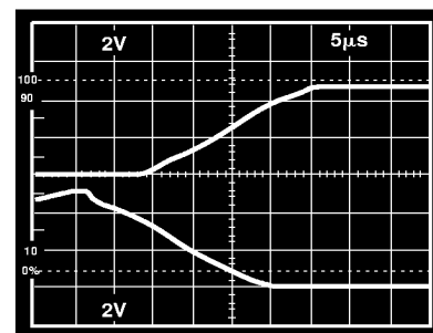
Figure 11. Precision Comparator
