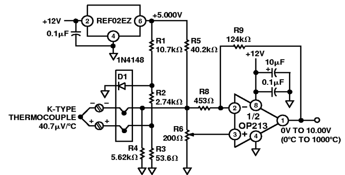
Figure 4. Accurate K-Type Thermocouple Amplifier
