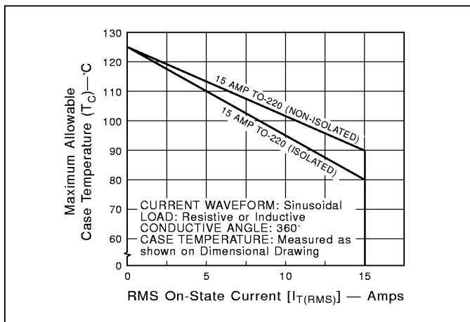
Figure 4.3 Maximum Allowable Case Temperature vs On-State Current (15 Amp Devices)
