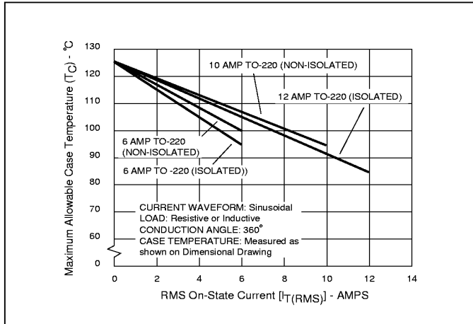
Figure 4.1 Maximum Allowable Case Temperature vs On-State Current (6-12 Amp Devices)
