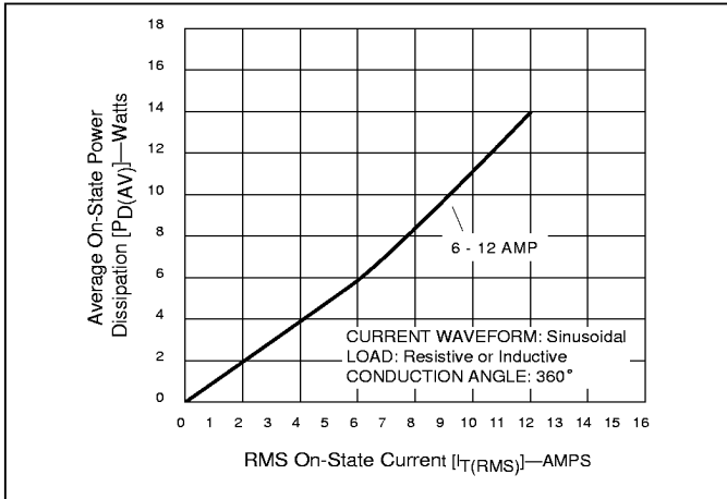
Figure 4.13 Power Dissipation (Typical) vs On-State Current (6-12 Amp Devices)
