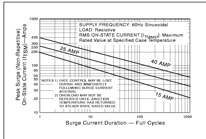
Figure 4.11 Peak Surge Current vs Surge Current Duration (15-40 Amp Devices)
