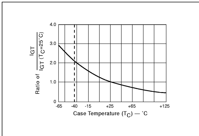
Figure 4.8 Normalized DC Gate Trigger Current for all Quadrants vs Case Temperature
