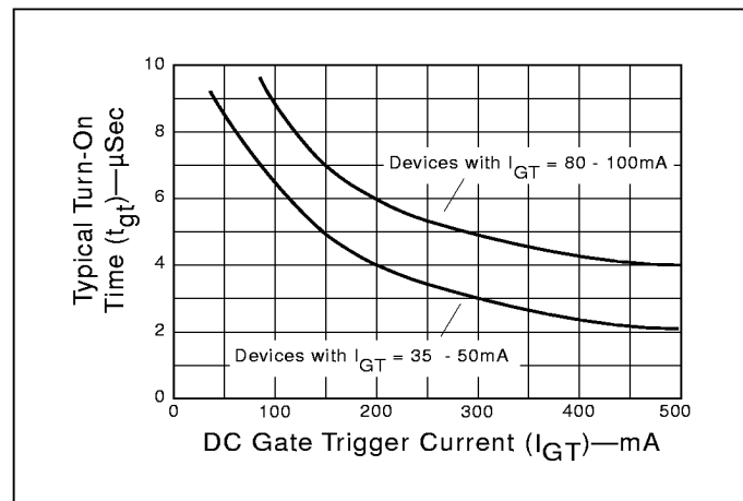
Figure 4.12 Turn-On Time vs Gate Trigger Current (Typical)
