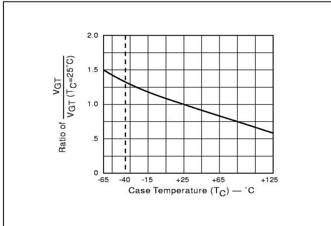
Figure 4.7 Normalized DC Gate Trigger Voltage for all Quadrants vs Case Temperature
