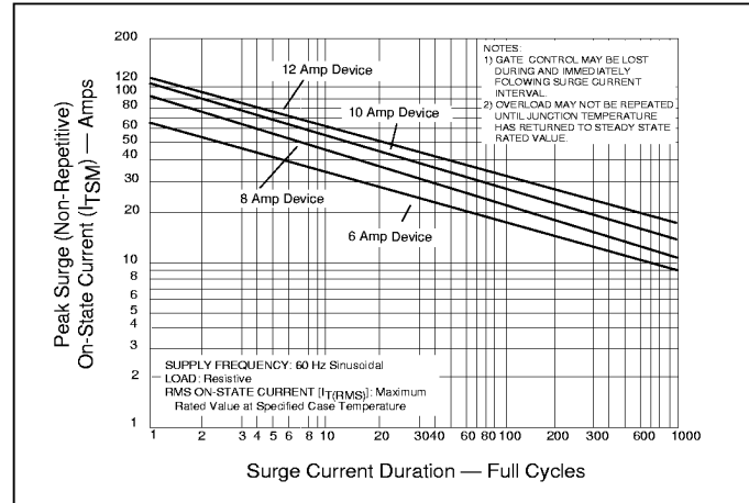
Figure 4.10 Peak Surge Current vs Surge Current Duration (6-12 Amp Devices)
