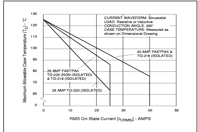
Figure 4.4 Maximum Allowable Case Temperature vs On-State Current (25 and 40 Amp Devices)
