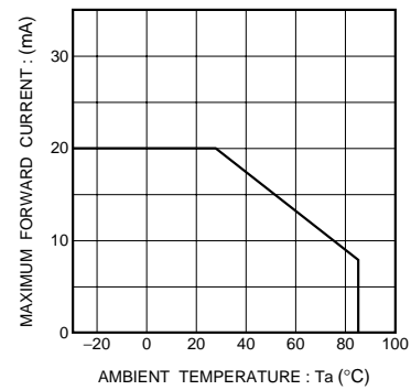
Fig.7 Derating
