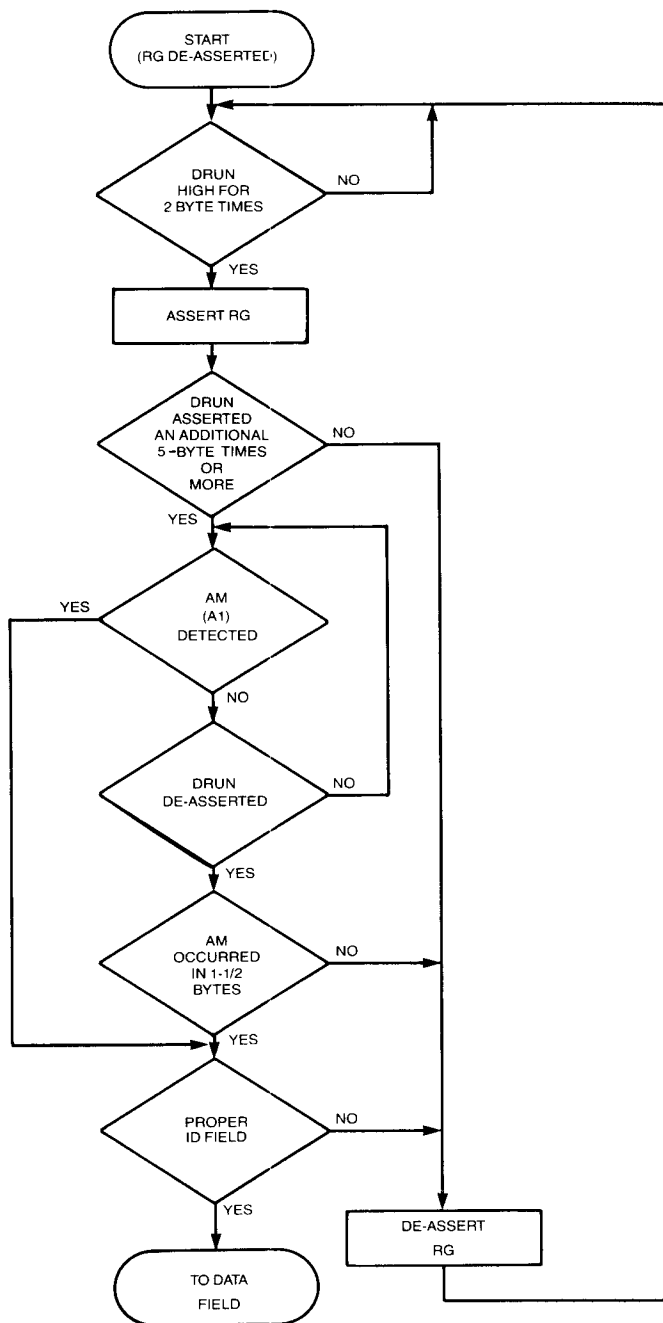
FIGURE 5. PLL CONTROL SEQUENCE FOR ID FIELD
