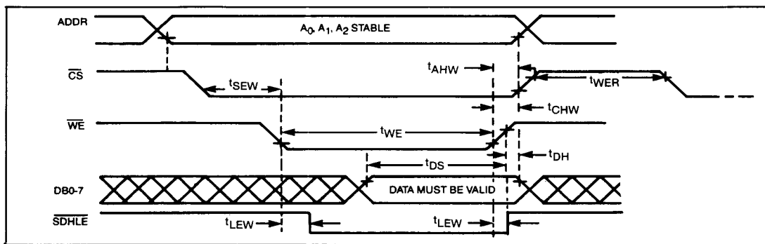
HOST WRITE TIMING
