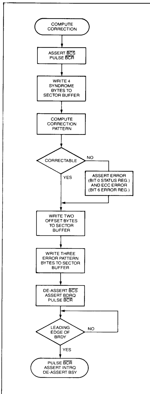
FIGURE 15. COMPUTE CORRECTION COMMAND
