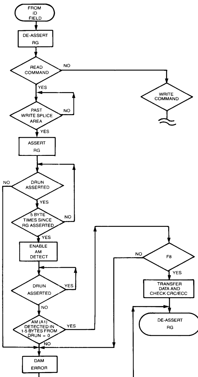
FIGURE 5A. PLL CONTROL SEQUENCE FOR DATA FIELD
