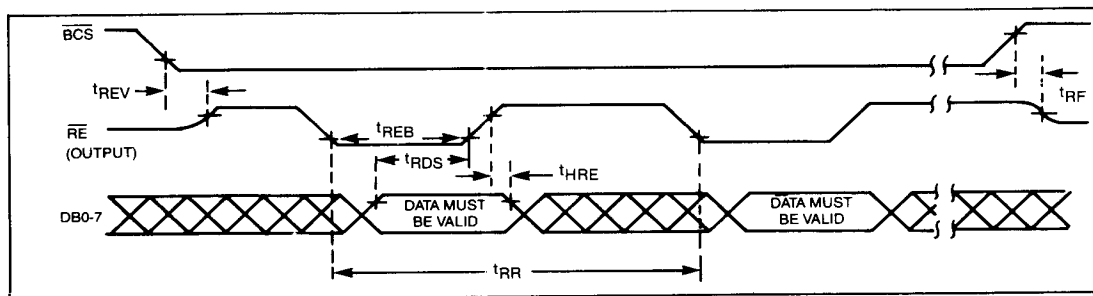
BUFFER READ TIMING
