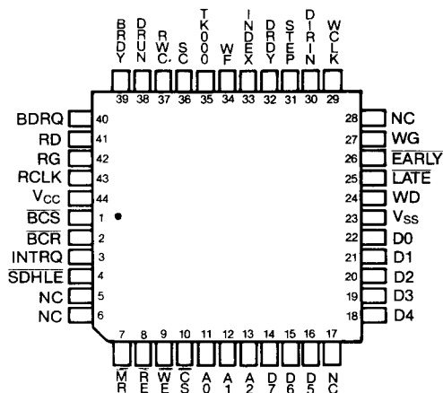
QUAD PIN DESIGNATION
