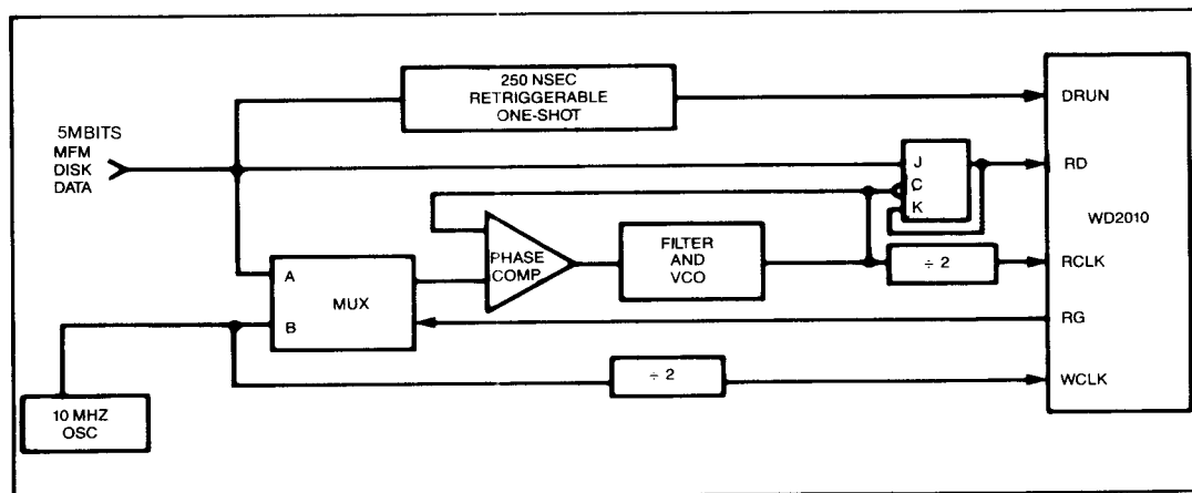
FIGURE 4. DATA SEPARATOR CIRCUIT
