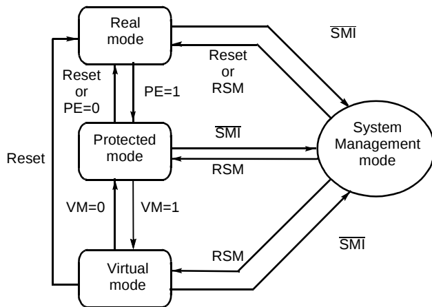
Figure 27. Transition to and from SMM
