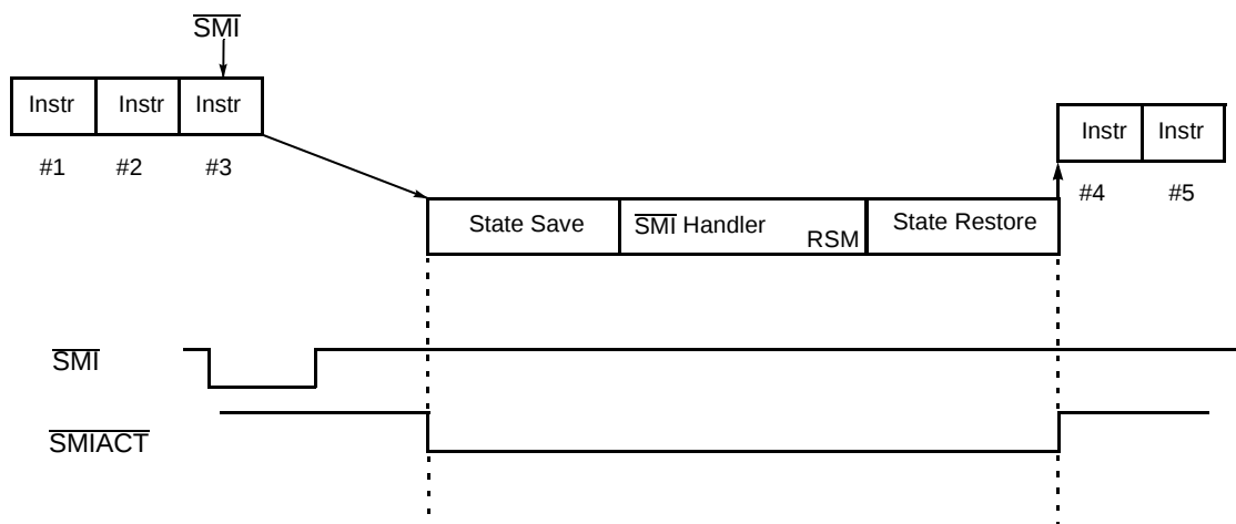
Figure 22. Basic \overline{\text{S}}\text{M}\text{I} Interrupt Service
