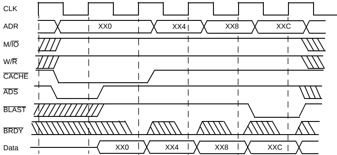
Figure 16. Burst Write
