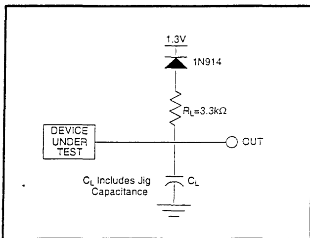
Figure 17. Transient Equivalent Testing Load Circuit
