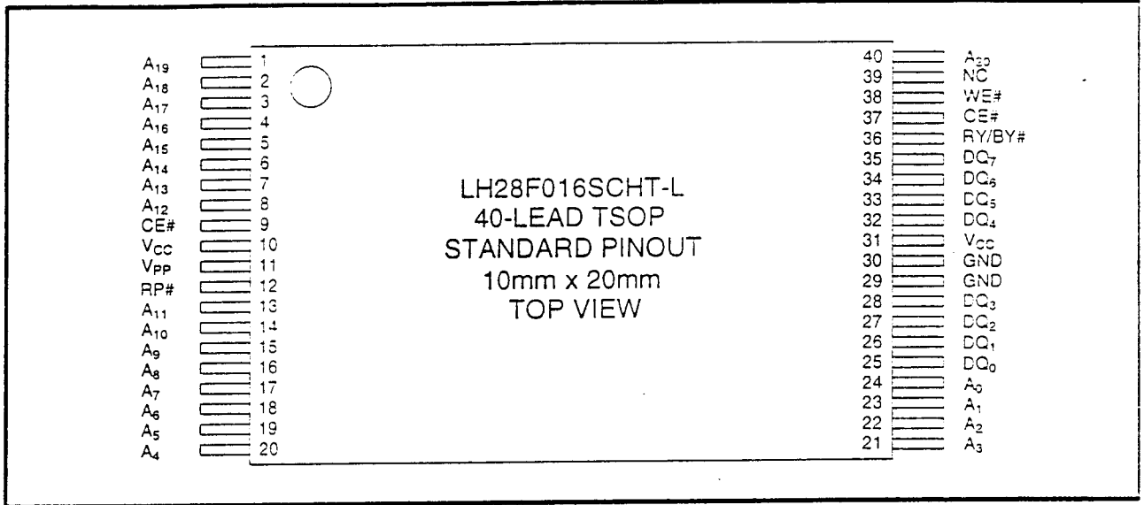
Figure 2. TSOP(Normal Bend) 40-Lead Pinout
