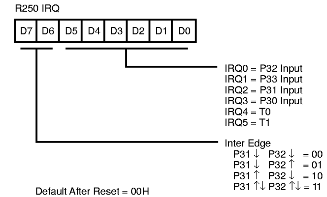
Figure 50. Interrupt Request Register FAH: Read/Write
