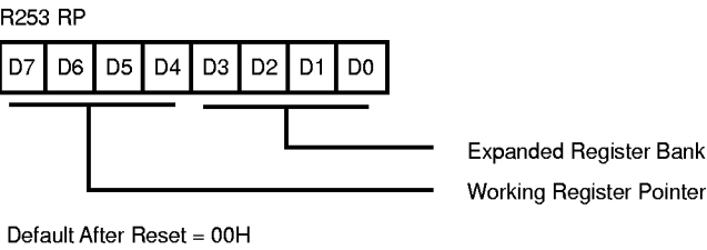
Figure 53. Register Pointer FDH: Read/Write
