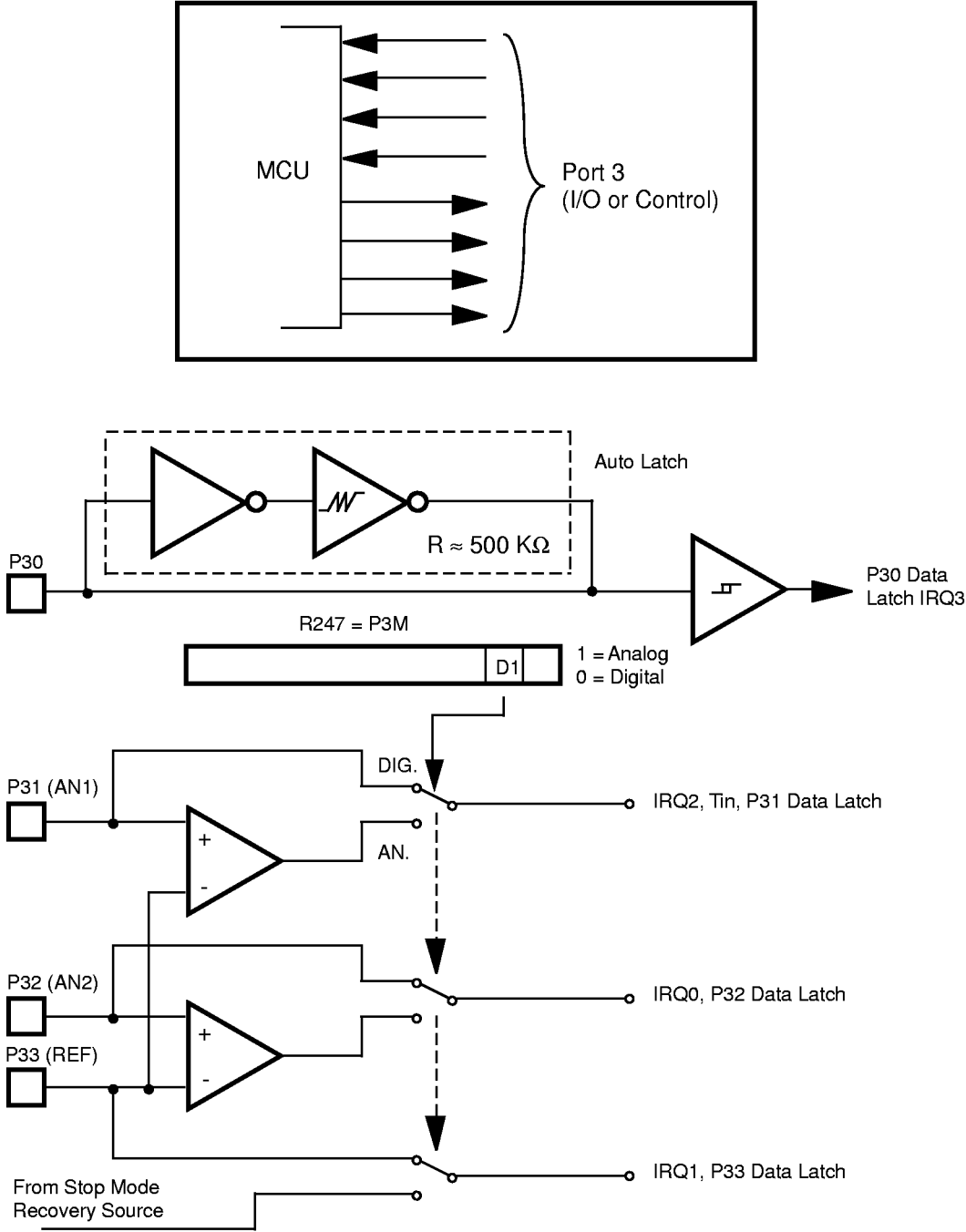
Figure 21. Port 3 Configuration
