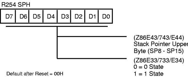
Figure 54. Stack Pointer High FEH: Read/Write
