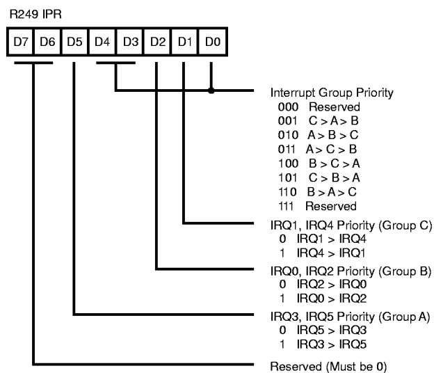
Figure 49. Interrupt Priority Register F9H: Write Only
