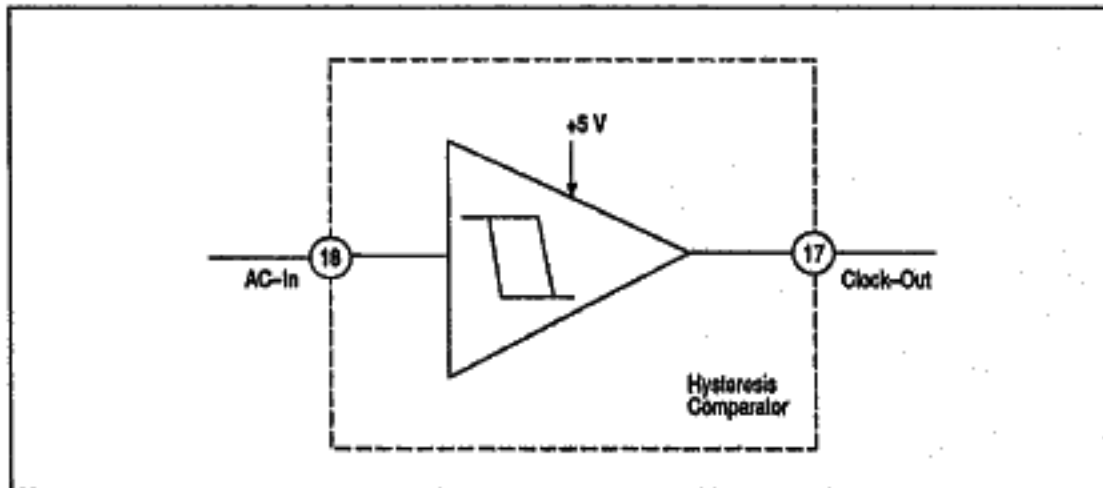
Figure 8 Hysteresis Comparator
