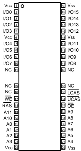
44(50) Pin Plastic TSOP-II
