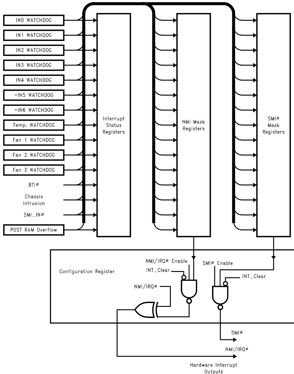
FIGURE 12. Interrupt Structure
