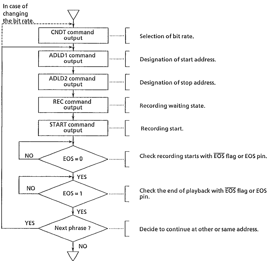
Fig.5.18 Recording procedure at the DIRECT MODE
