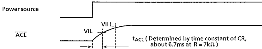
Fig. 5.31 \overline{ACL} input at power on reset
