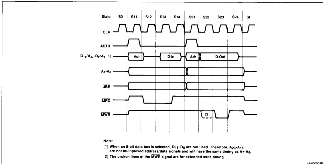
Figure 30. Memory-to-Memory Transfer
