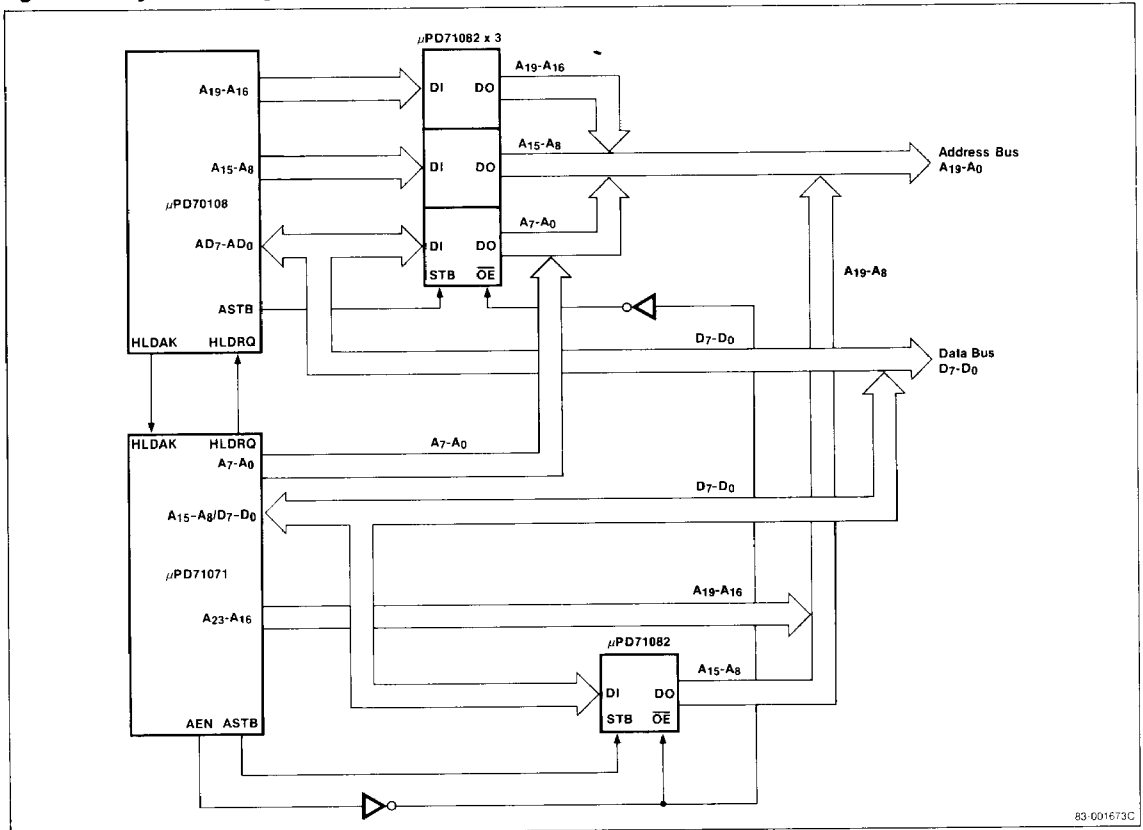
Figure 32. System Configuration with μPD71018
