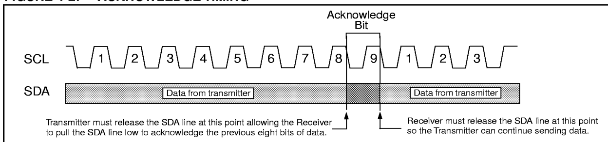
FIGURE 4-2: ACKNOWLEDGE TIMING
