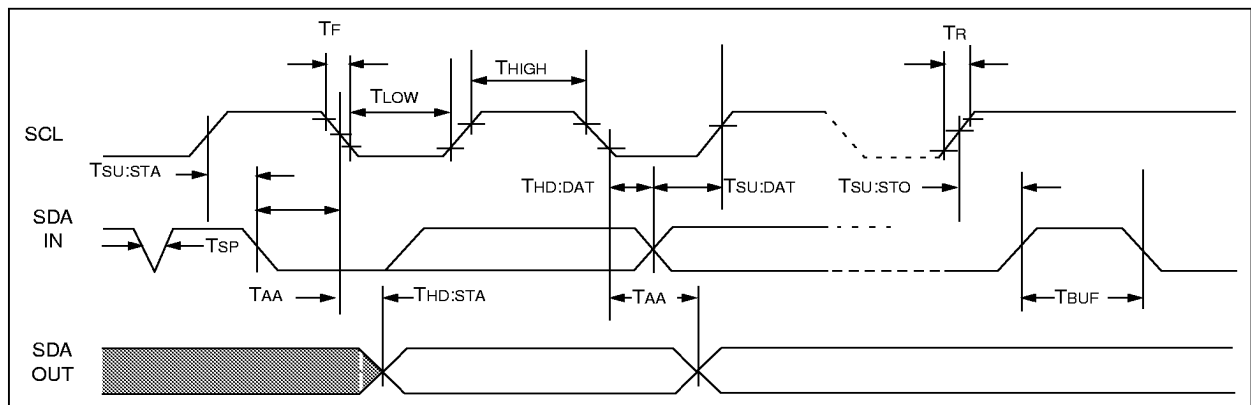
FIGURE 1-1: BUSTIMING DATA
