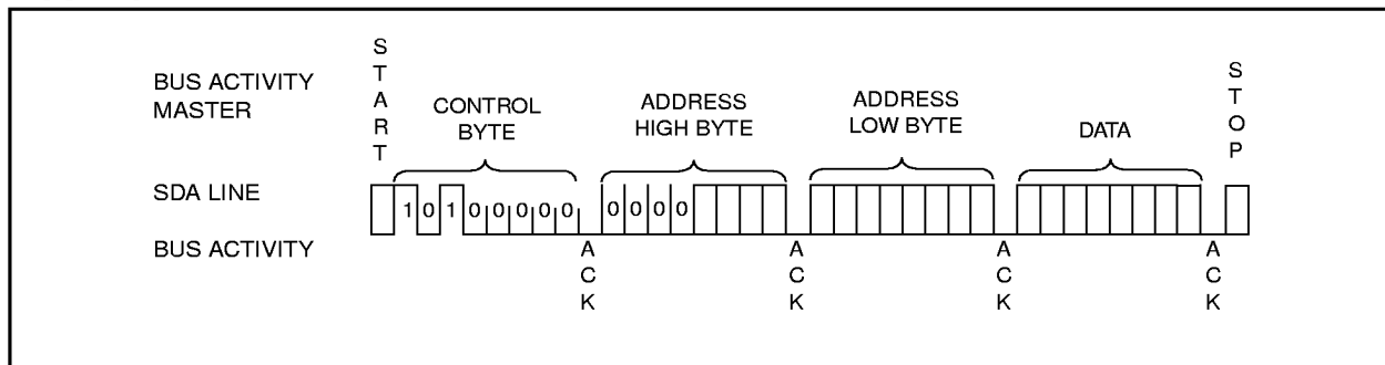
FIGURE 6-1: BYTE WRITE
