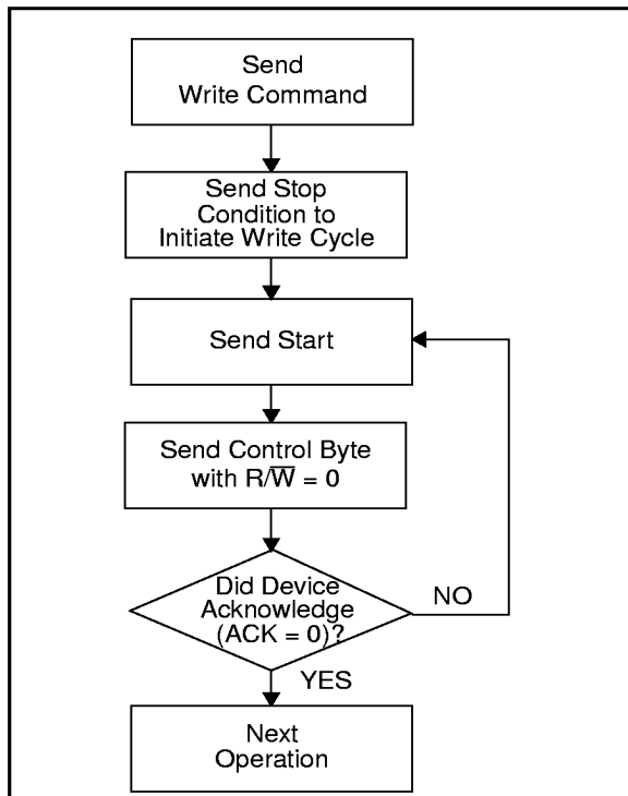
FIGURE 7-1: ACKNOWLEDGE POLLING FLOW
