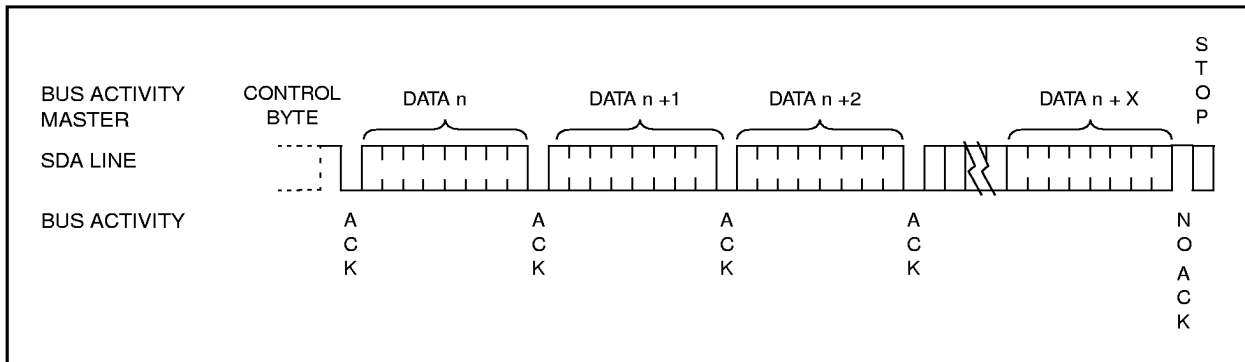
FIGURE 8-3: SEQUENTIAL READ
