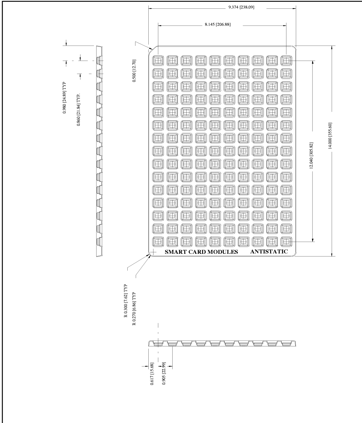
FIGURE 9-1: TRAY DIMENSIONS
