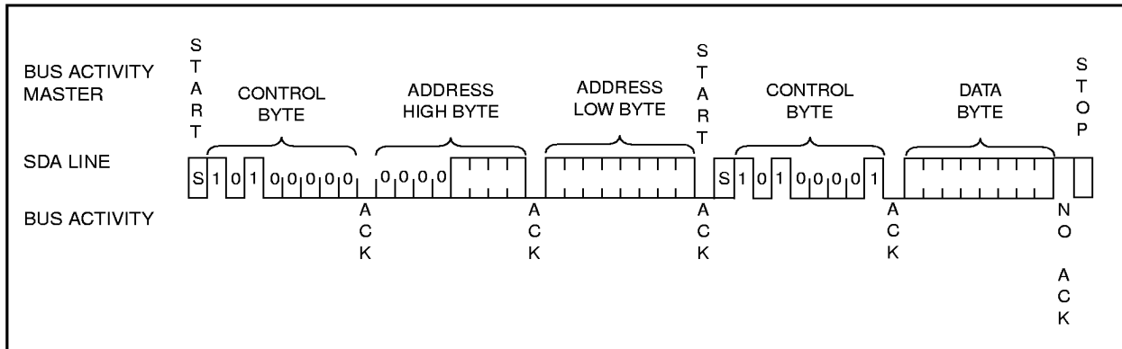
FIGURE 8-2: RANDOM READ
