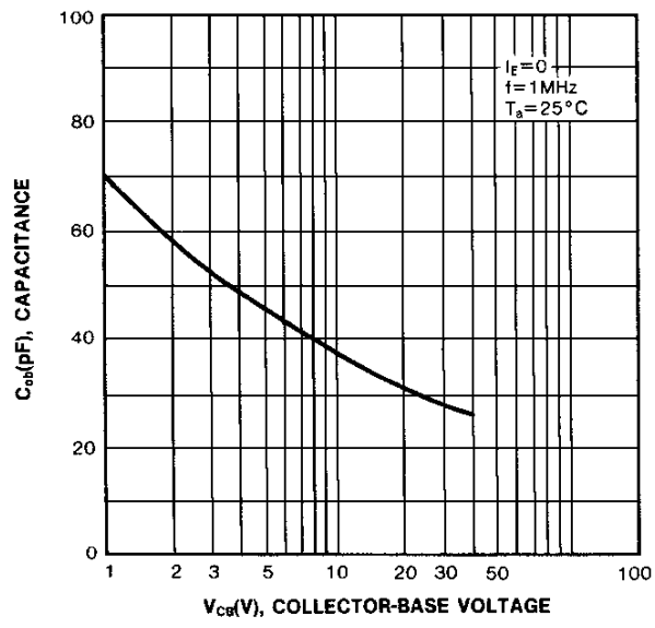
OUTPUT CAPACITANCE
