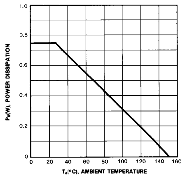
POWER DERATING
