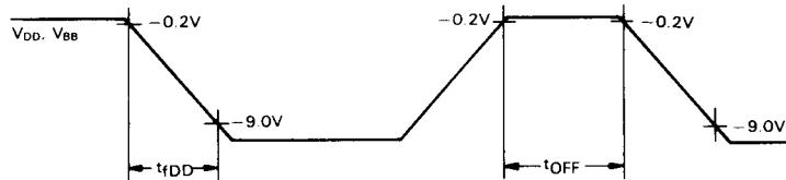
Figure 22 Power Supply Timing for Built-in Reset Circuit
