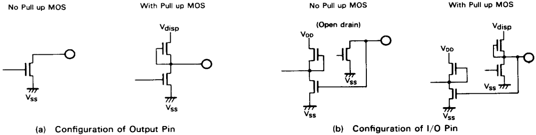
Figure 17 I/O Configuration
