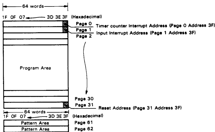
Figure 2 ROM Address Space
