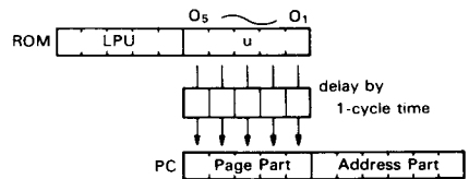
Figure 8 LPU Operation
