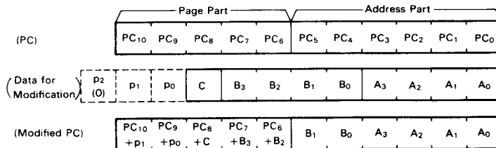
Figure 9 Modification of Program Counter by TBR Instruction
