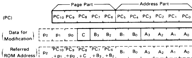
Figure 5 ROM Addressing for Pattern Generation
