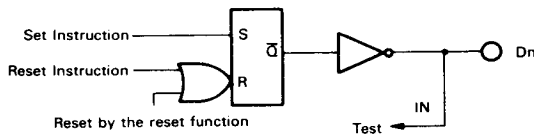
Figure 15 1-bit Discrete I/O Block Diagram
