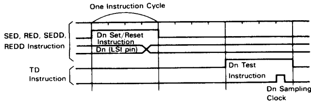
Figure 16 1-bit Discrete I/O Timing
