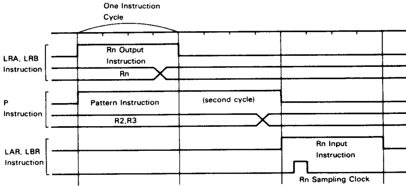
Figure 14 4-bit Data I/O Timing
