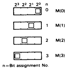
Figure 12 RAM Bit and Operand n
