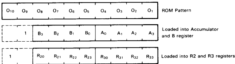
Figure 6 Correspondence of Each Bit of Pattern
