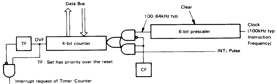
Figure 18 Timer/Counter Block Diagram
