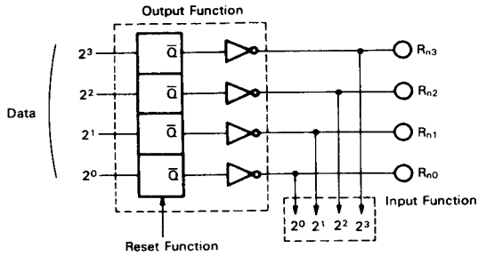
Figure 13 4-bit Data I/O Block Diagram
