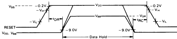
Figure 23 Data Hold Timing
