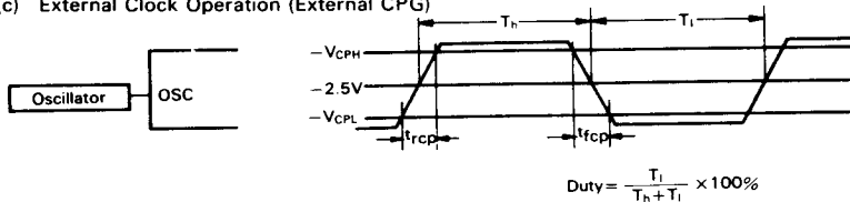
Figure 24 Clock Operation Mode
