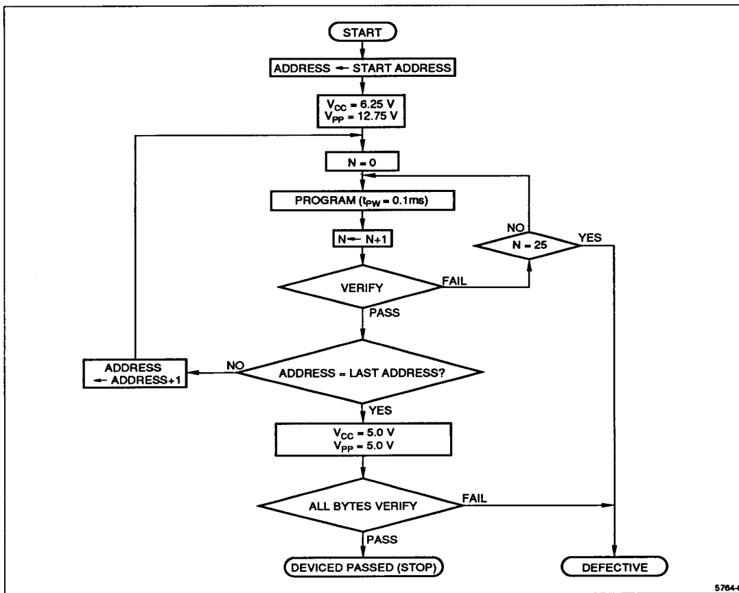
Figure 6. Programming Flowchart
