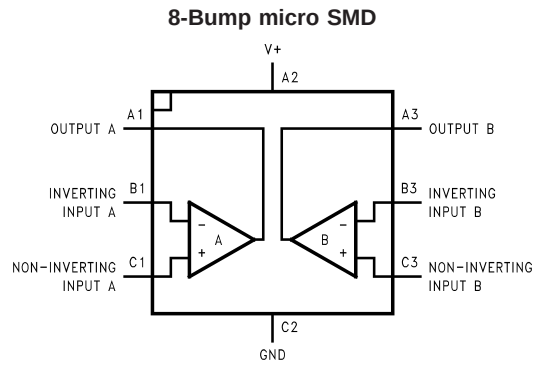
Top View (Bump Side Down)
