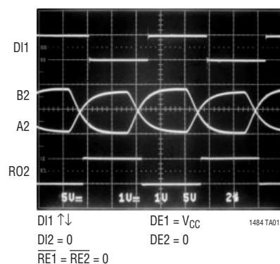
Driving a 2000 Foot STP Cable
