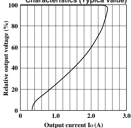
Fig.4 Overcurrent Protection Characteristics (Typica value)
