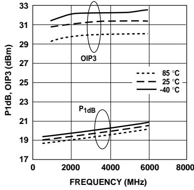
Figure 15. P_{1dB} , IP_3 vs. Frequency and Temperature at V_{DS} = 4\text{ V} , I_{DS} = 60\text{ mA} . [1]
