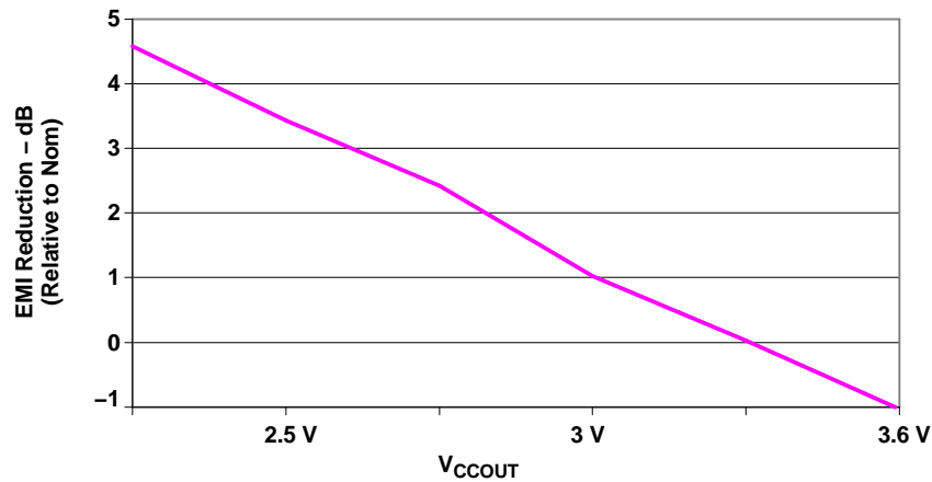
Figure 17. EMI Reduction vs V ccout
