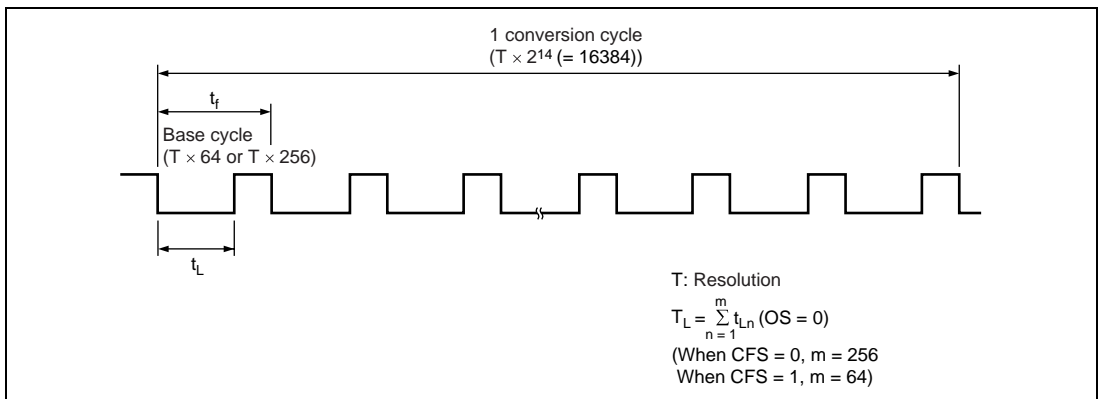
Figure 10.2 PWM D/A Operation
