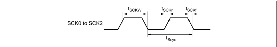
Figure 28.23 SCK Clock Input Timing
