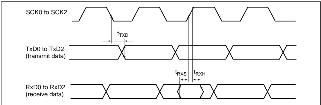
Figure 28.24 SCI Input/Output Timing (Synchronous Mode)
