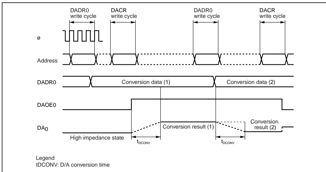
Figure 20.2 D/A Converter Operation Example
