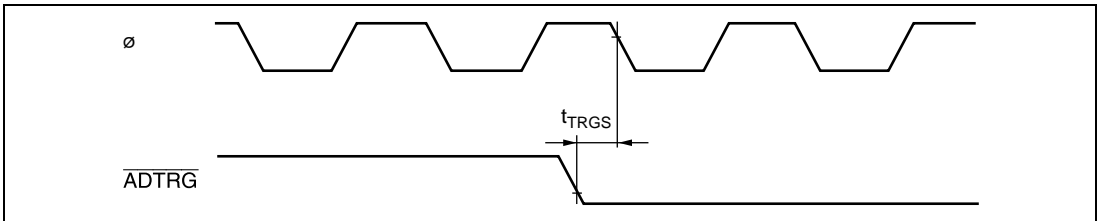
Figure 28.25 A/D Converter External Trigger Input Timing
