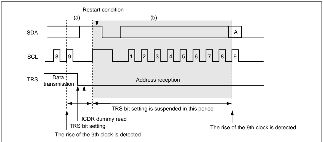
Figure 16.35 TRS Bit Set Timing in Slave Mode
