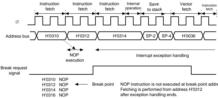
Figure 5.10 Address Break Timing Example
