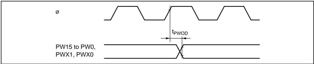
Figure 28.22 PWM, PWMX Output Timing
