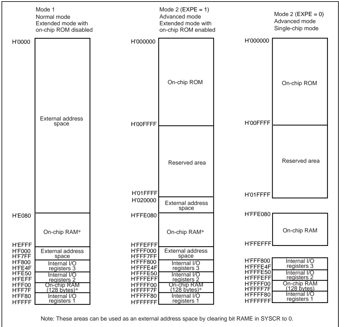
Figure 3.1 Address Map for H8S/2140B and H8S/2160B (1)
