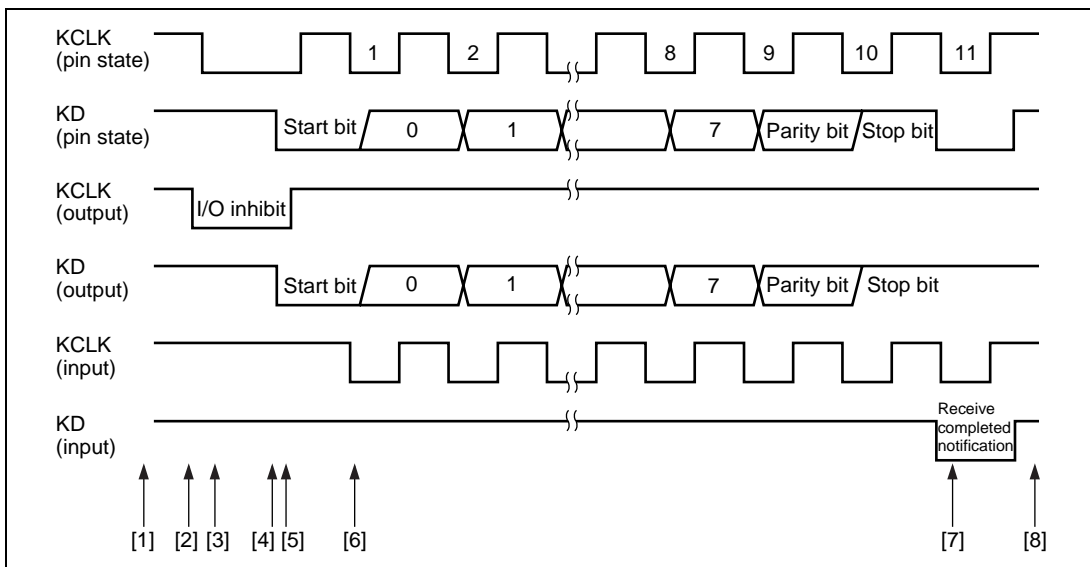
Figure 17.6 Transmit Timing
