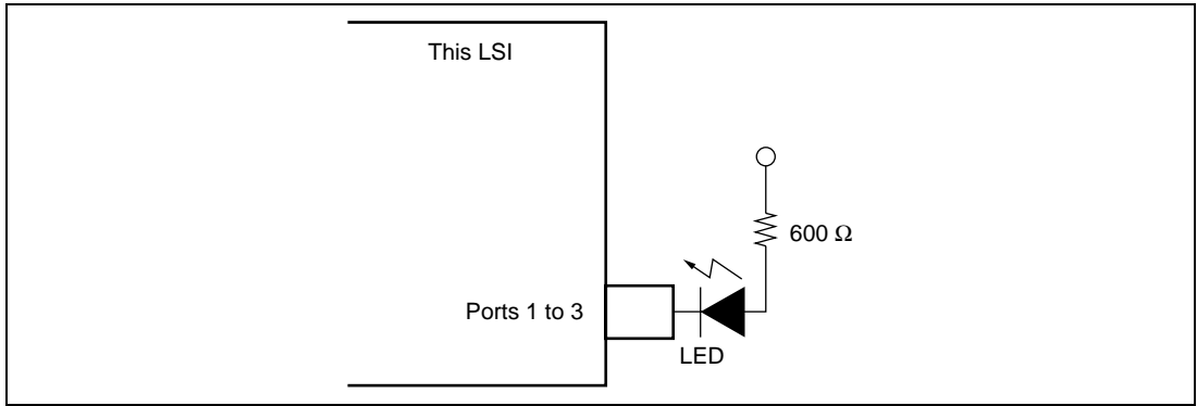
Figure 28.2 LED Drive Circuit (Example)
