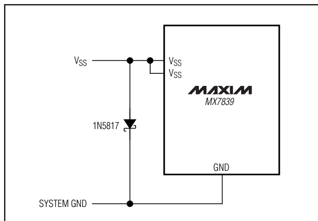
Figure 3. Schottky Diode Between V_{SS} and GND
