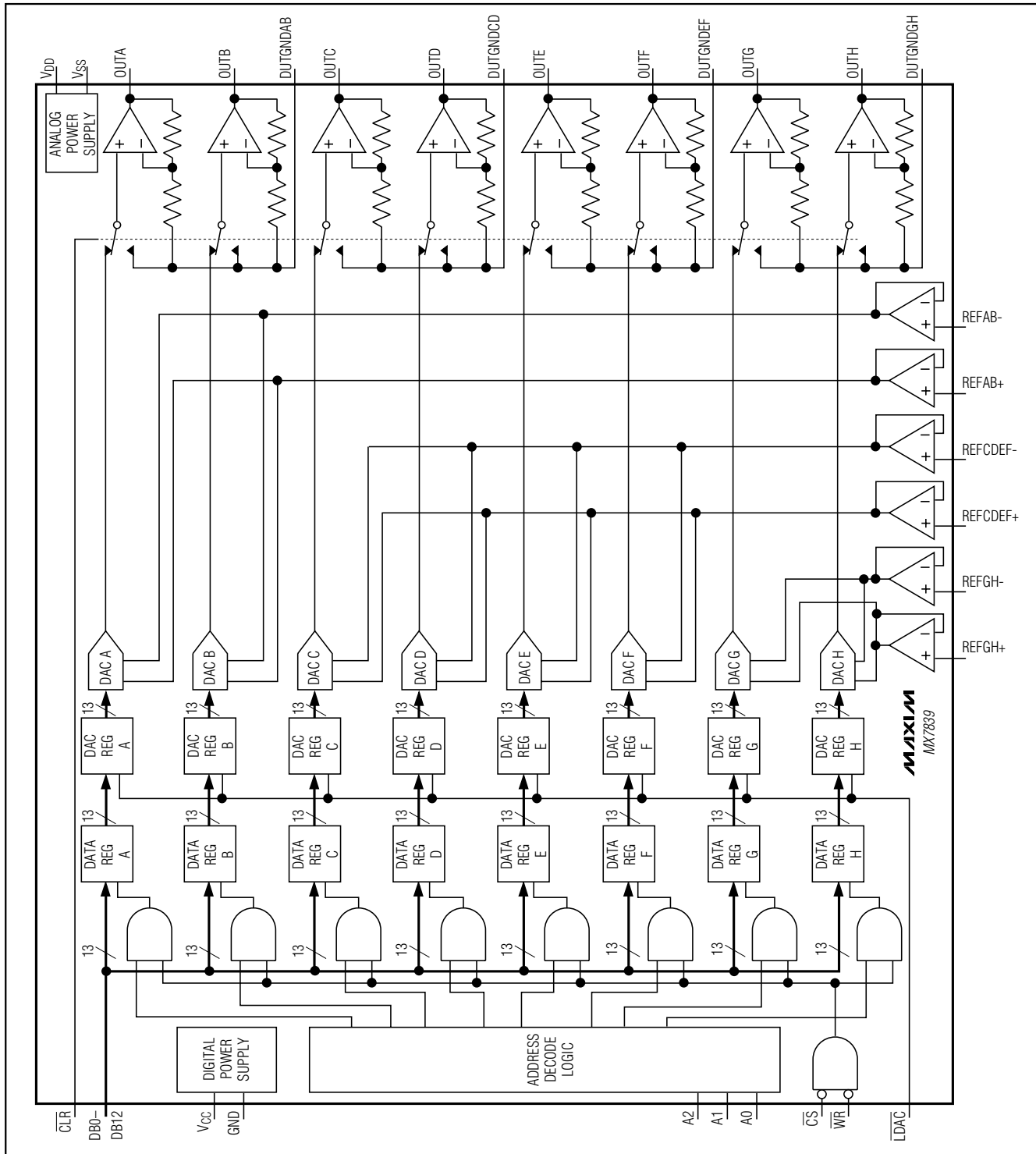
Functional Diagram
